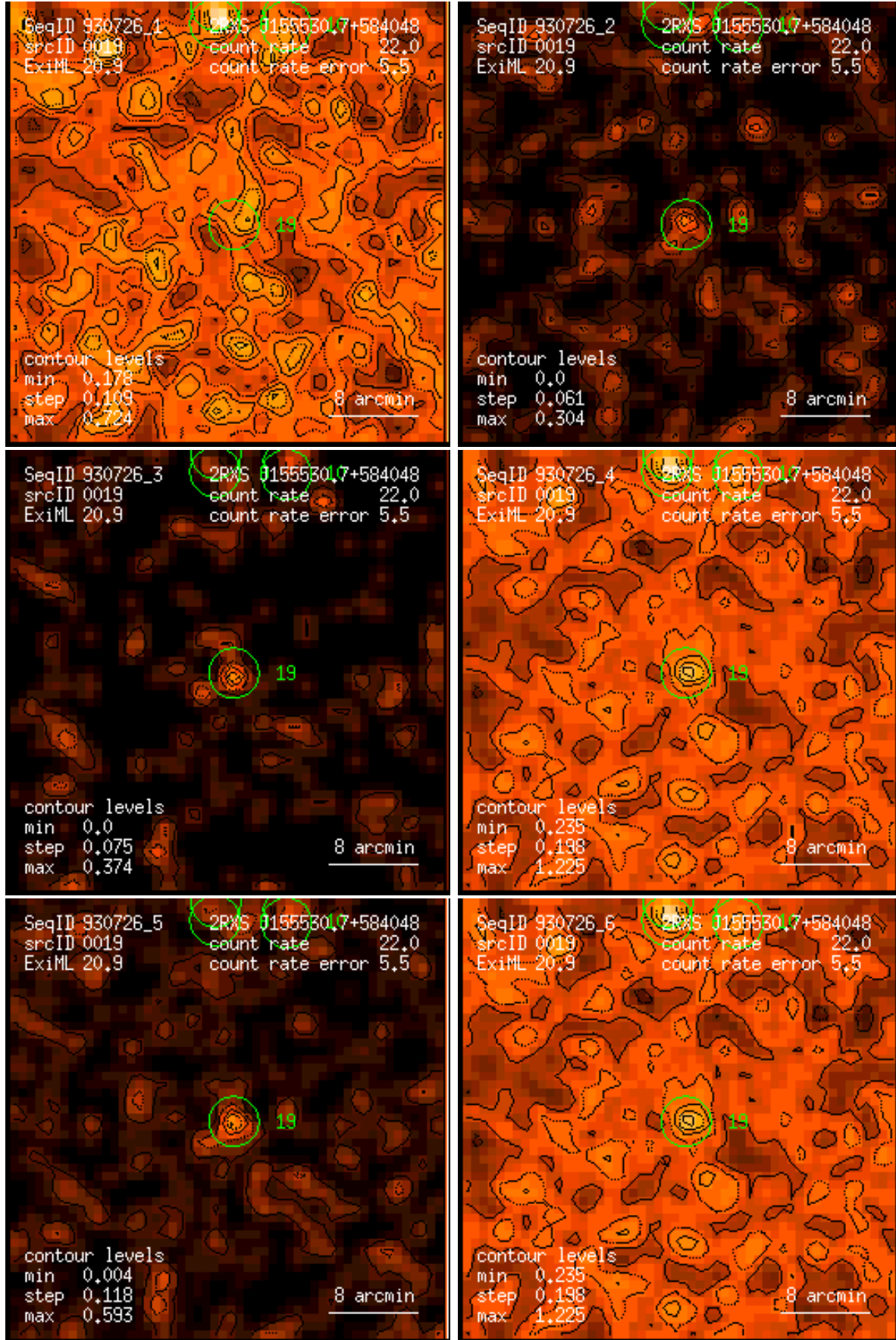
Figure 19: RASS 930726: detection 0019: band rate images, Gaussian filter: (1) PSPC channels 11 – 41, (2) 52 – 90, (3) 91 – 201, (4) 11 – 235, (5) 52 – 201, (6) 11 – 201. Broad band rates in counts/ks. Band rate contour levels in counts/ks/arcmin 2 .
