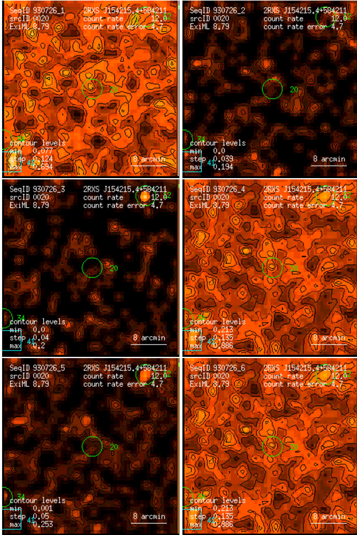
Figure 20: RASS 930726: detection 0020: band rate images, Gaussian filter: (1) PSPC channels 11 – 41, (2) 52 – 90, (3) 91 – 201, (4) 11 – 235, (5) 52 – 201, (6) 11 – 201. Broad band rates in counts/ks. Band rate contour levels in counts/ks/arcmin 2 .
