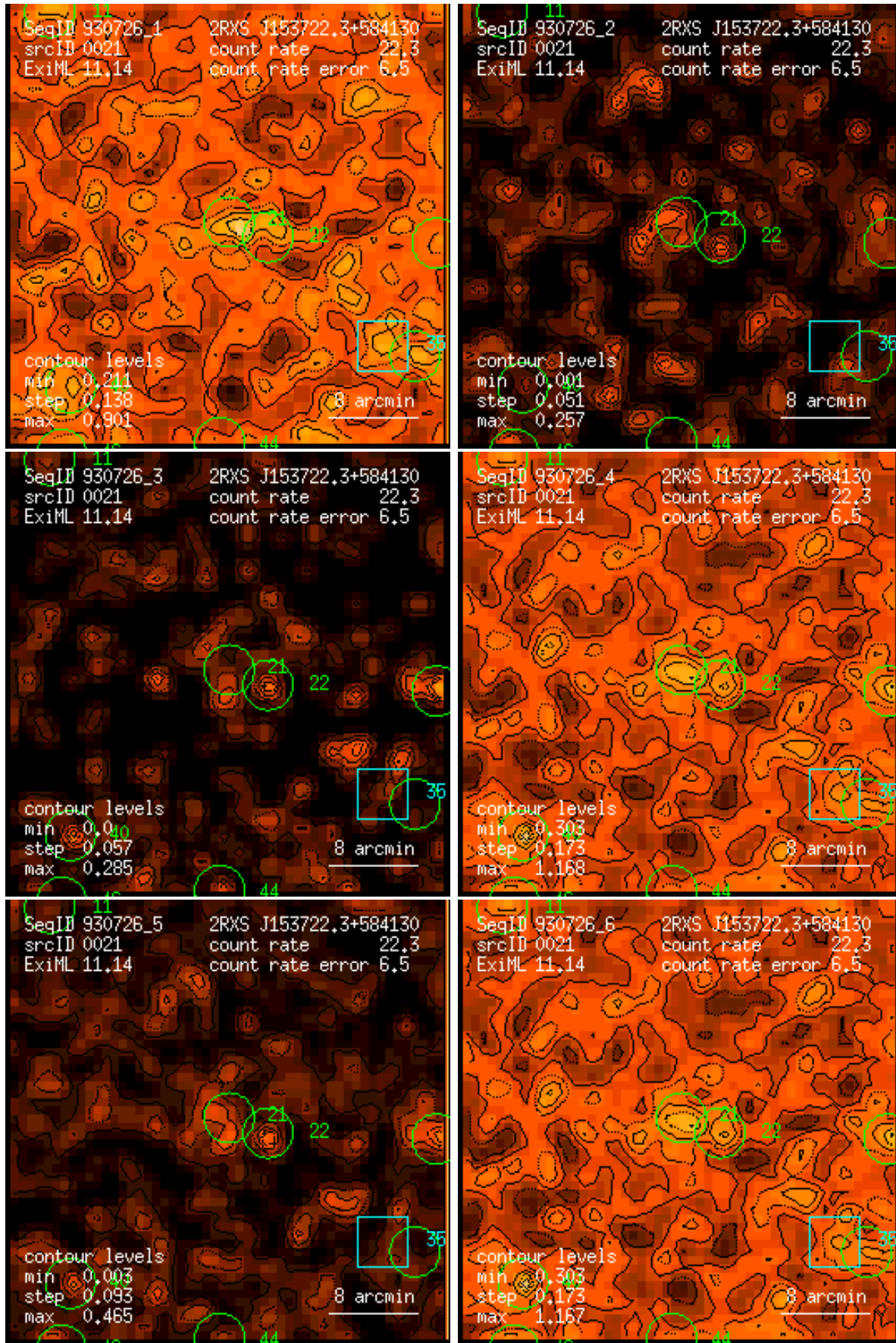
Figure 21: RASS 930726: detection 0021: band rate images, Gaussian filter: (1) PSPC channels 11 – 41, (2) 52 – 90, (3) 91 – 201, (4) 11 – 235, (5) 52 – 201, (6) 11 – 201. Broad band rates in counts/ks. Band rate contour levels in counts/ks/arcmin 2 .
