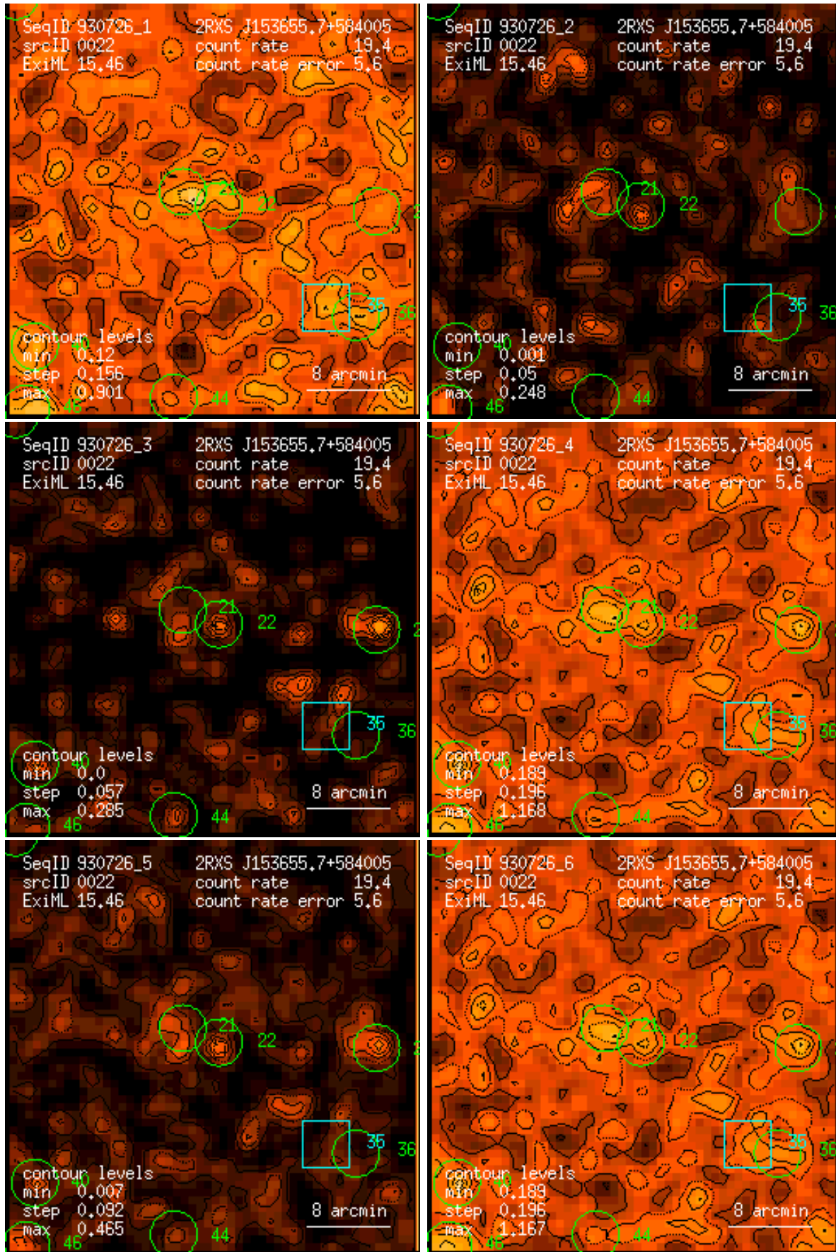
Figure 22: RASS 930726: detection 0022: band rate images, Gaussian filter: (1) PSPC channels 11 – 41, (2) 52 – 90, (3) 91 – 201, (4) 11 – 235, (5) 52 – 201, (6) 11 – 201. Broad band rates in counts/ks. Band rate contour levels in counts/ks/arcmin 2 .
