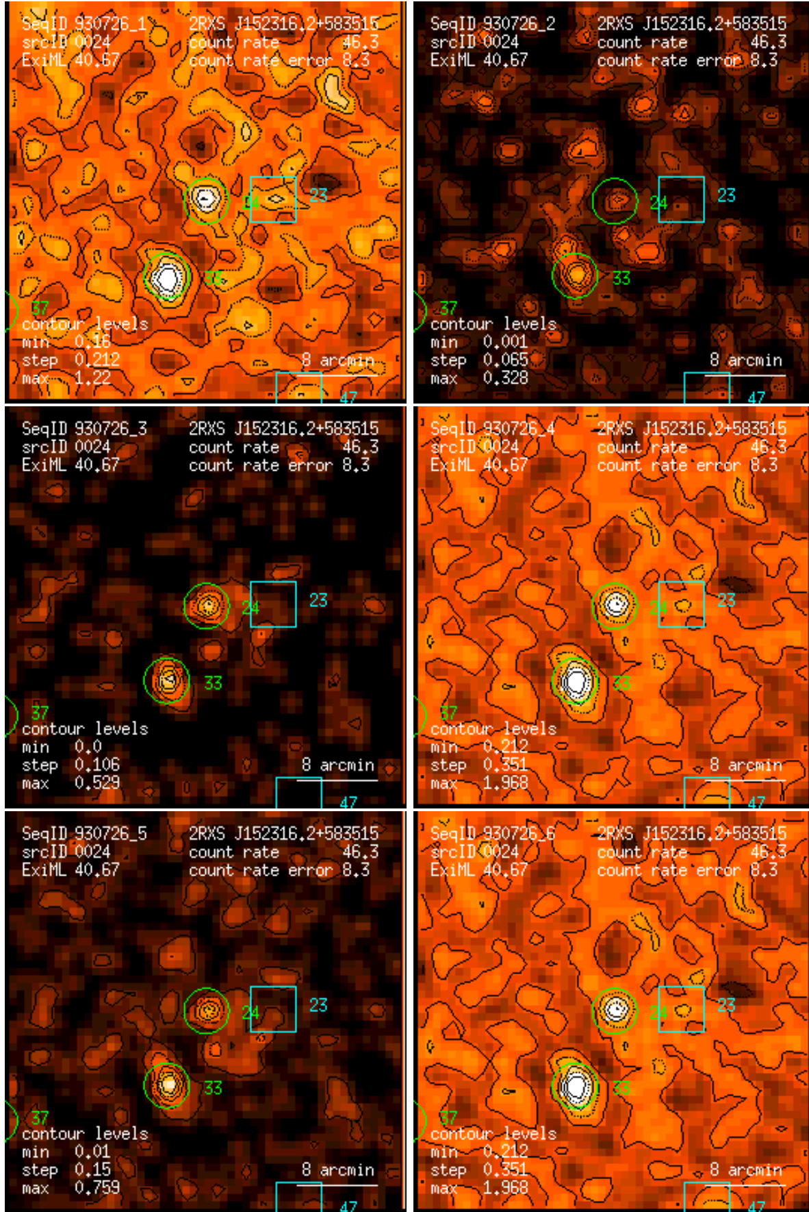
Figure 24: RASS 930726: detection 0024: band rate images, Gaussian filter: (1) PSPC channels 11 – 41, (2) 52 – 90, (3) 91 – 201, (4) 11 – 235, (5) 52 – 201, (6) 11 – 201. Broad band rates in counts/ks. Band rate contour levels in counts/ks/arcmin 2 .
