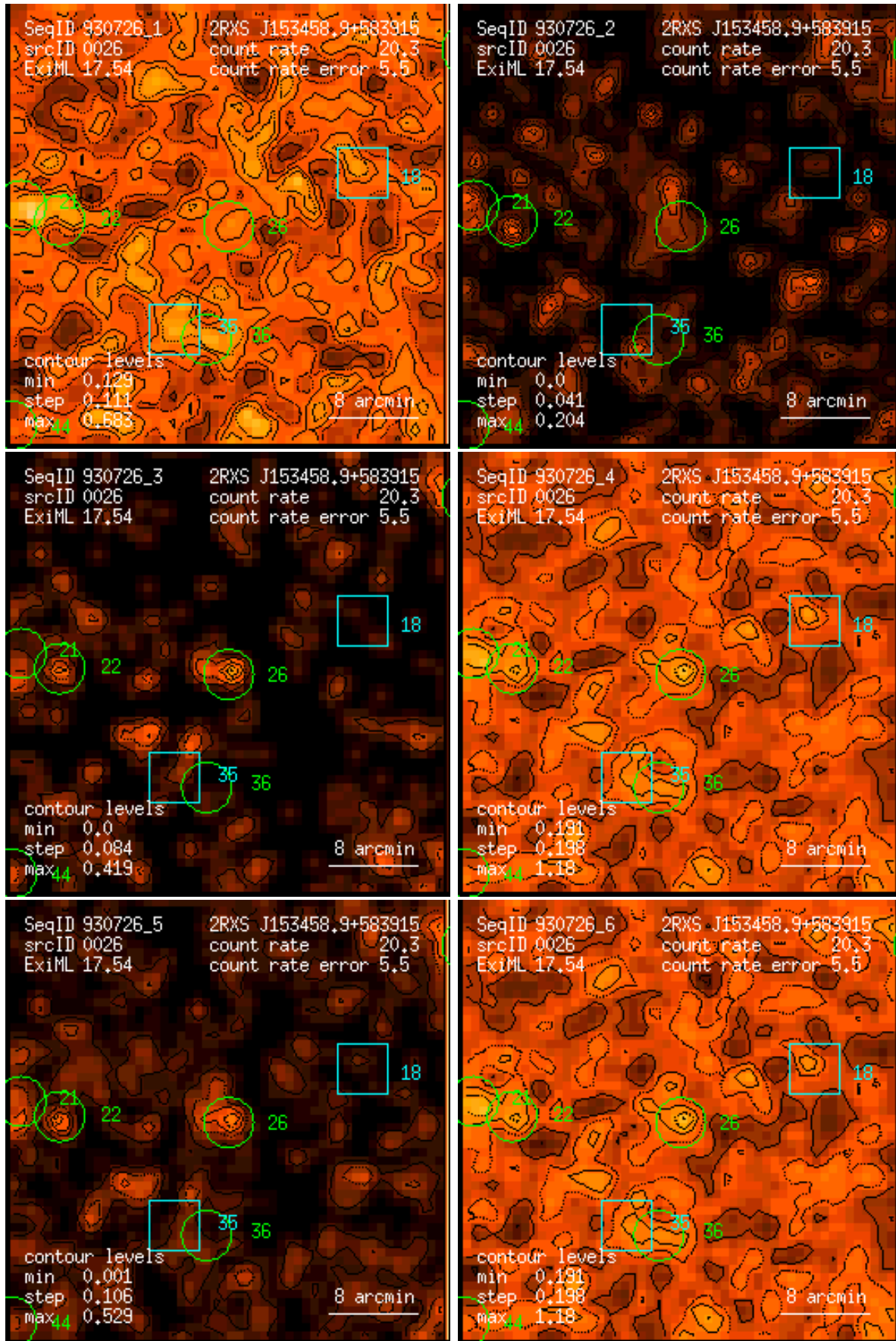
Figure 26: RASS 930726: detection 0026: band rate images, Gaussian filter: (1) PSPC channels 11 – 41, (2) 52 – 90, (3) 91 – 201, (4) 11 – 235, (5) 52 – 201, (6) 11 – 201. Broad band rates in counts/ks. Band rate contour levels in counts/ks/arcmin 2 .
