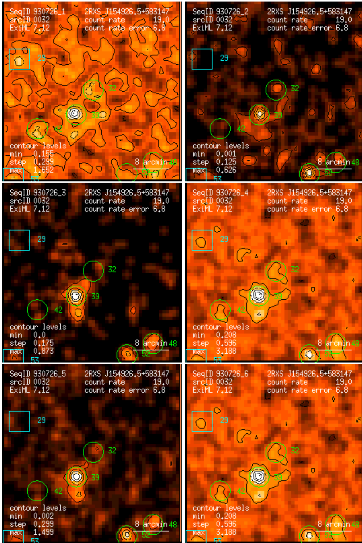
Figure 32: RASS 930726: detection 0032: band rate images, Gaussian filter: (1) PSPC channels 11 – 41, (2) 52 – 90, (3) 91 – 201, (4) 11 – 235, (5) 52 – 201, (6) 11 – 201. Broad band rates in counts/ks. Band rate contour levels in counts/ks/arcmin 2 .
