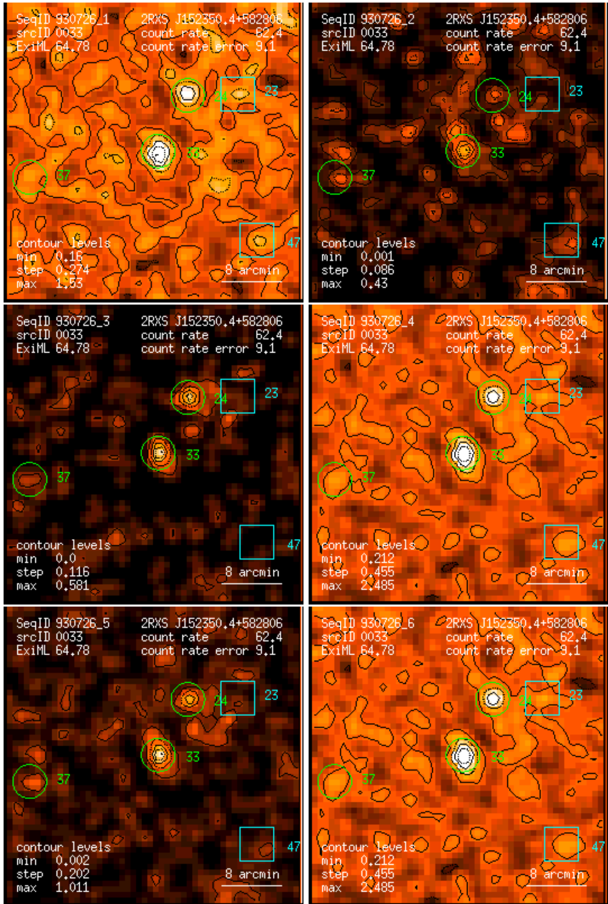
Figure 33: RASS 930726: detection 0033: band rate images, Gaussian filter: (1) PSPC channels 11 – 41, (2) 52 – 90, (3) 91 – 201, (4) 11 – 235, (5) 52 – 201, (6) 11 – 201. Broad band rates in counts/ks. Band rate contour levels in counts/ks/arcmin 2 .
