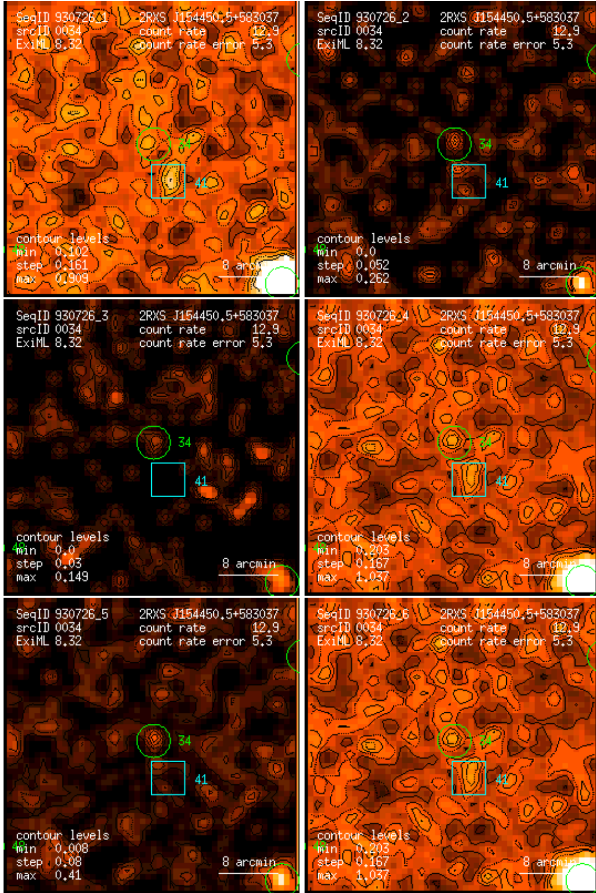
Figure 34: RASS 930726: detection 0034: band rate images, Gaussian filter: (1) PSPC channels 11 – 41, (2) 52 – 90, (3) 91 – 201, (4) 11 – 235, (5) 52 – 201, (6) 11 – 201. Broad band rates in counts/ks. Band rate contour levels in counts/ks/arcmin 2 .
