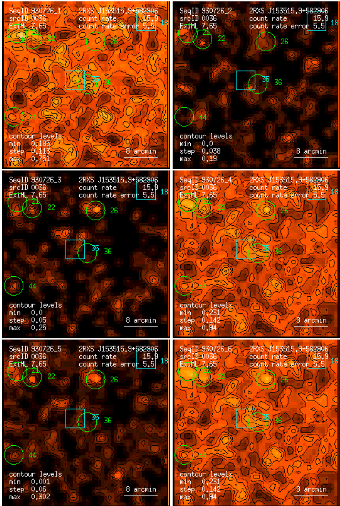
Figure 36: RASS 930726: detection 0036: band rate images, Gaussian filter: (1) PSPC channels 11 – 41, (2) 52 – 90, (3) 91 – 201, (4) 11 – 235, (5) 52 – 201, (6) 11 – 201. Broad band rates in counts/ks. Band rate contour levels in counts/ks/arcmin 2 .
