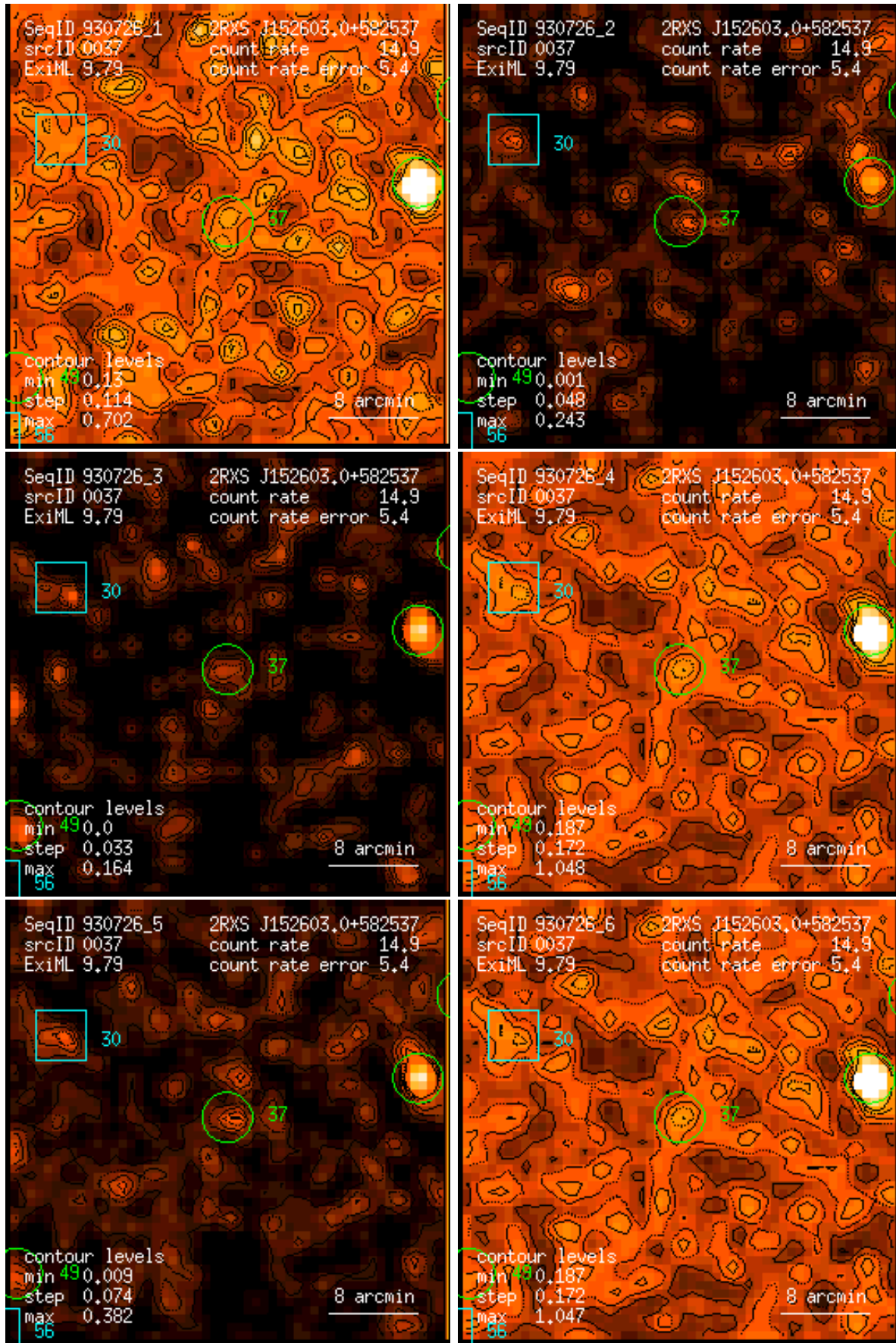
Figure 37: RASS 930726: detection 0037: band rate images, Gaussian filter: (1) PSPC channels 11 – 41, (2) 52 – 90, (3) 91 – 201, (4) 11 – 235, (5) 52 – 201, (6) 11 – 201. Broad band rates in counts/ks. Band rate contour levels in counts/ks/arcmin 2 .
