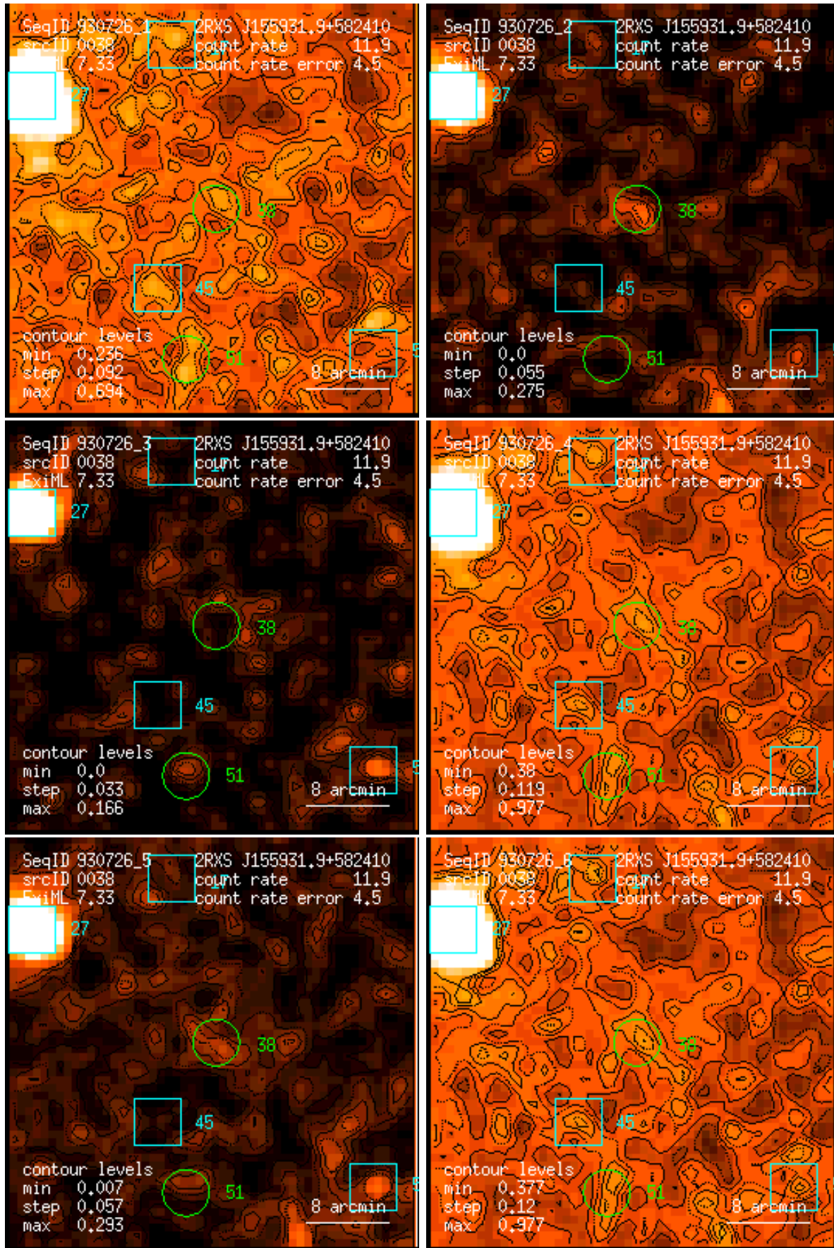
Figure 38: RASS 930726: detection 0038: band rate images, Gaussian filter: (1) PSPC channels 11 – 41, (2) 52 – 90, (3) 91 – 201, (4) 11 – 235, (5) 52 – 201, (6) 11 – 201. Broad band rates in counts/ks. Band rate contour levels in counts/ks/arcmin 2 .
