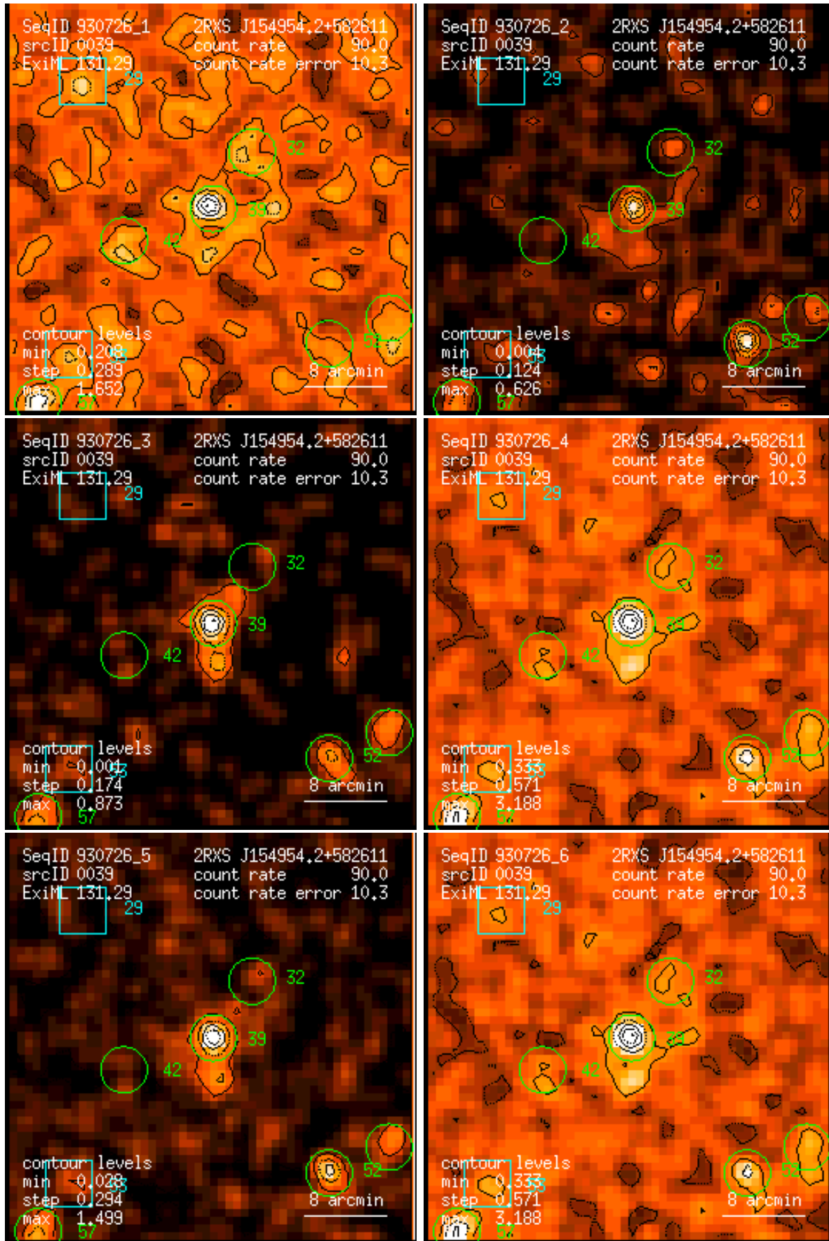
Figure 39: RASS 930726: detection 0039: band rate images, Gaussian filter: (1) PSPC channels 11 – 41, (2) 52 – 90, (3) 91 – 201, (4) 11 – 235, (5) 52 – 201, (6) 11 – 201. Broad band rates in counts/ks. Band rate contour levels in counts/ks/arcmin 2 .
