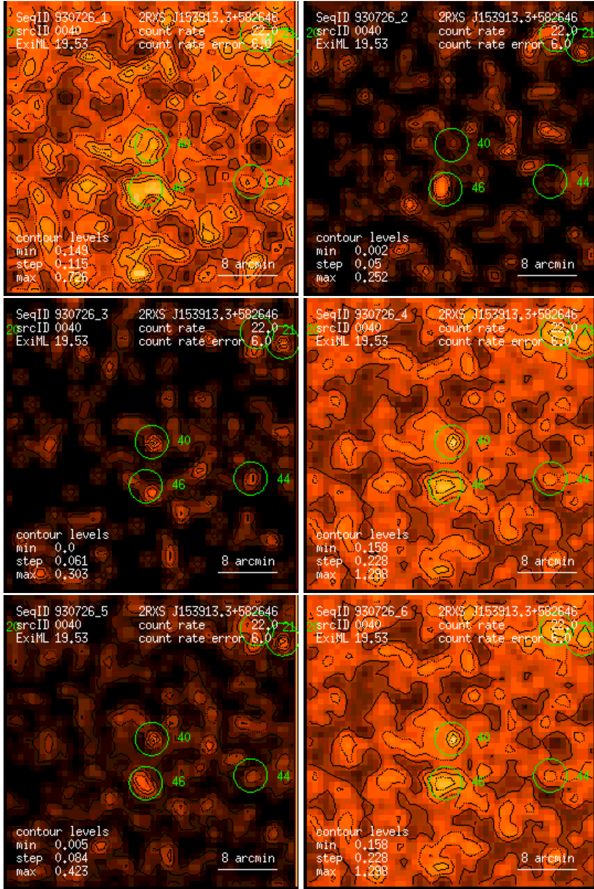
Figure 40: RASS 930726: detection 0040: band rate images, Gaussian filter: (1) PSPC channels 11 – 41, (2) 52 – 90, (3) 91 – 201, (4) 11 – 235, (5) 52 – 201, (6) 11 – 201. Broad band rates in counts/ks. Band rate contour levels in counts/ks/arcmin 2 .
