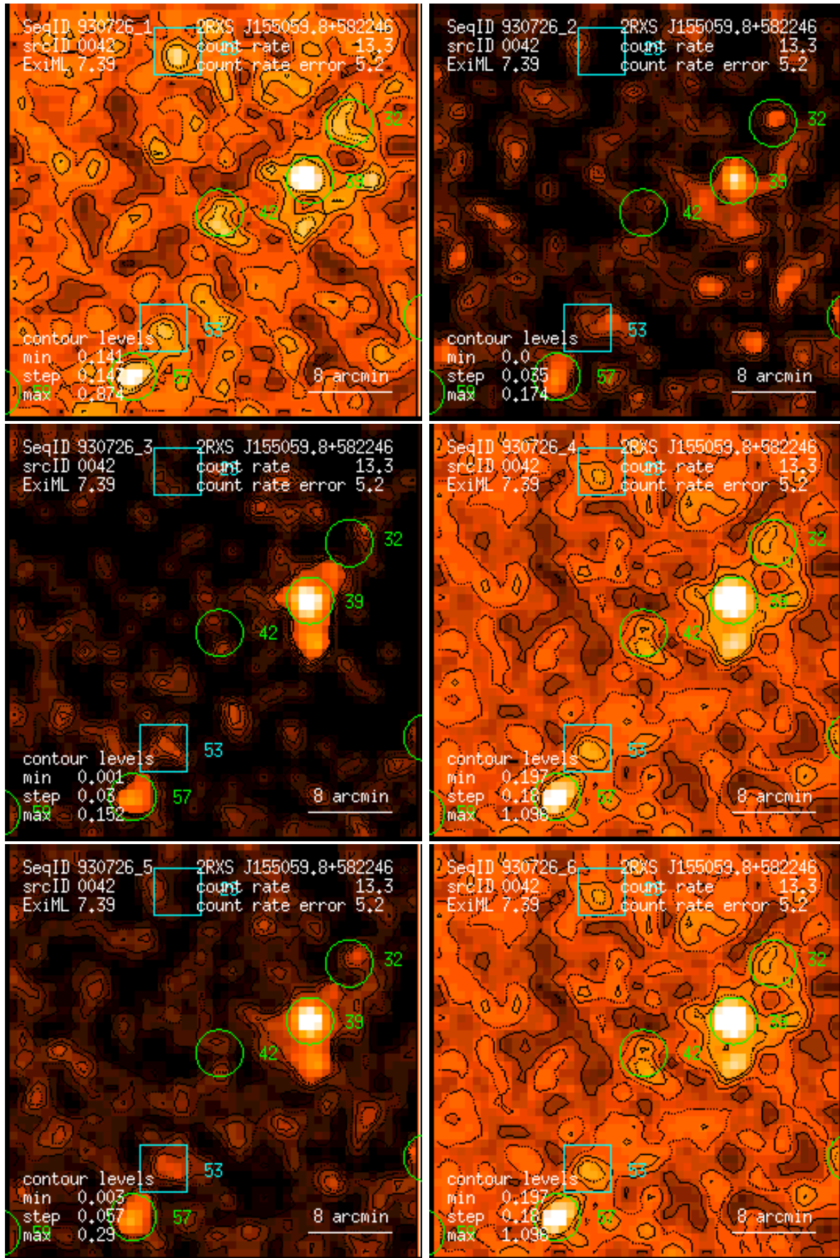
Figure 42: RASS 930726: detection 0042: band rate images, Gaussian filter: (1) PSPC channels 11 – 41, (2) 52 – 90, (3) 91 – 201, (4) 11 – 235, (5) 52 – 201, (6) 11 – 201. Broad band rates in counts/ks. Band rate contour levels in counts/ks/arcmin 2 .
