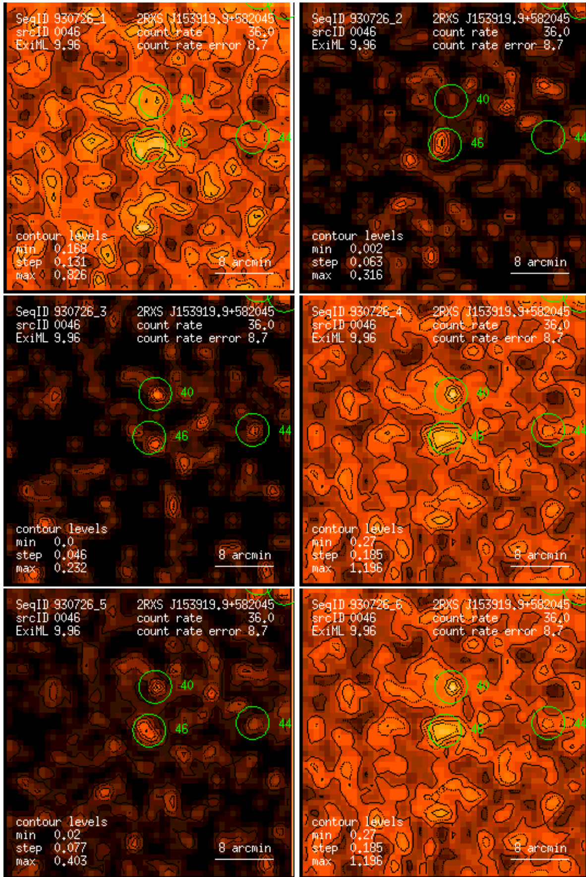
Figure 46: RASS 930726: detection 0046: band rate images, Gaussian filter: (1) PSPC channels 11 – 41, (2) 52 – 90, (3) 91 – 201, (4) 11 – 235, (5) 52 – 201, (6) 11 – 201. Broad band rates in counts/ks. Band rate contour levels in counts/ks/arcmin 2 .
