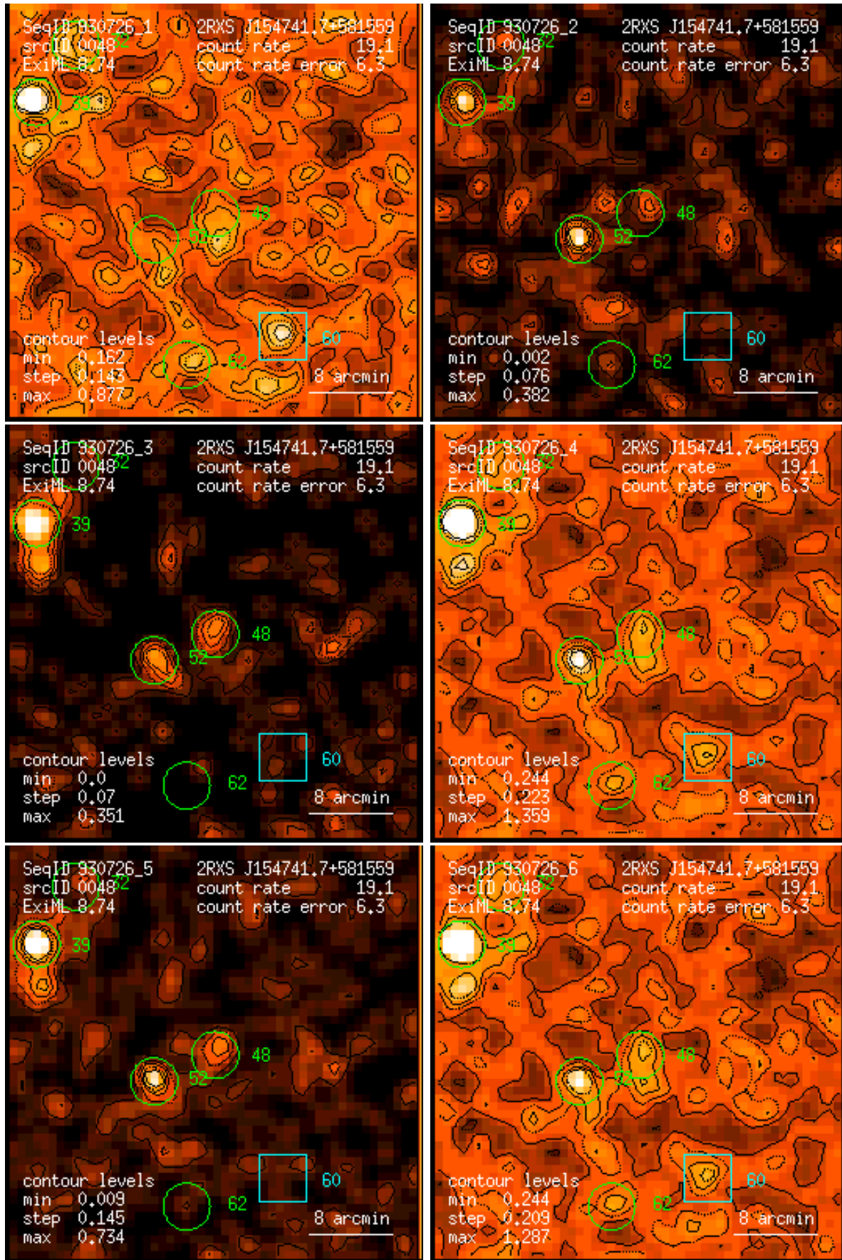
Figure 48: RASS 930726: detection 0048: band rate images, Gaussian filter: (1) PSPC channels 11 – 41, (2) 52 – 90, (3) 91 – 201, (4) 11 – 235, (5) 52 – 201, (6) 11 – 201. Broad band rates in counts/ks. Band rate contour levels in counts/ks/arcmin 2 .
