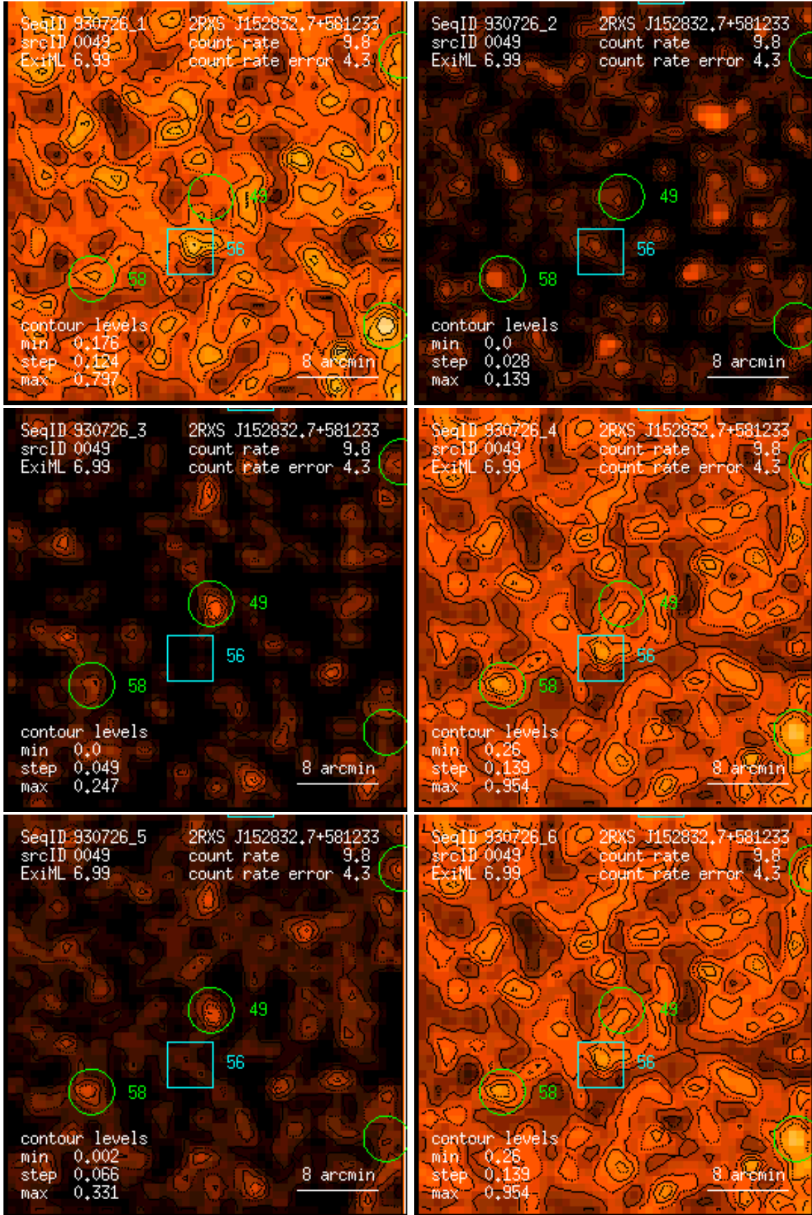
Figure 49: RASS 930726: detection 0049: band rate images, Gaussian filter: (1) PSPC channels 11 – 41, (2) 52 – 90, (3) 91 – 201, (4) 11 – 235, (5) 52 – 201, (6) 11 – 201. Broad band rates in counts/ks. Band rate contour levels in counts/ks/arcmin 2 .
