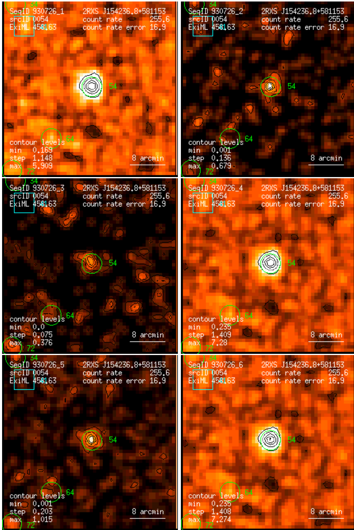
Figure 54: RASS 930726: detection 0054: band rate images, Gaussian filter: (1) PSPC channels 11 – 41, (2) 52 – 90, (3) 91 – 201, (4) 11 – 235, (5) 52 – 201, (6) 11 – 201. Broad band rates in counts/ks. Band rate contour levels in counts/ks/arcmin 2 .
