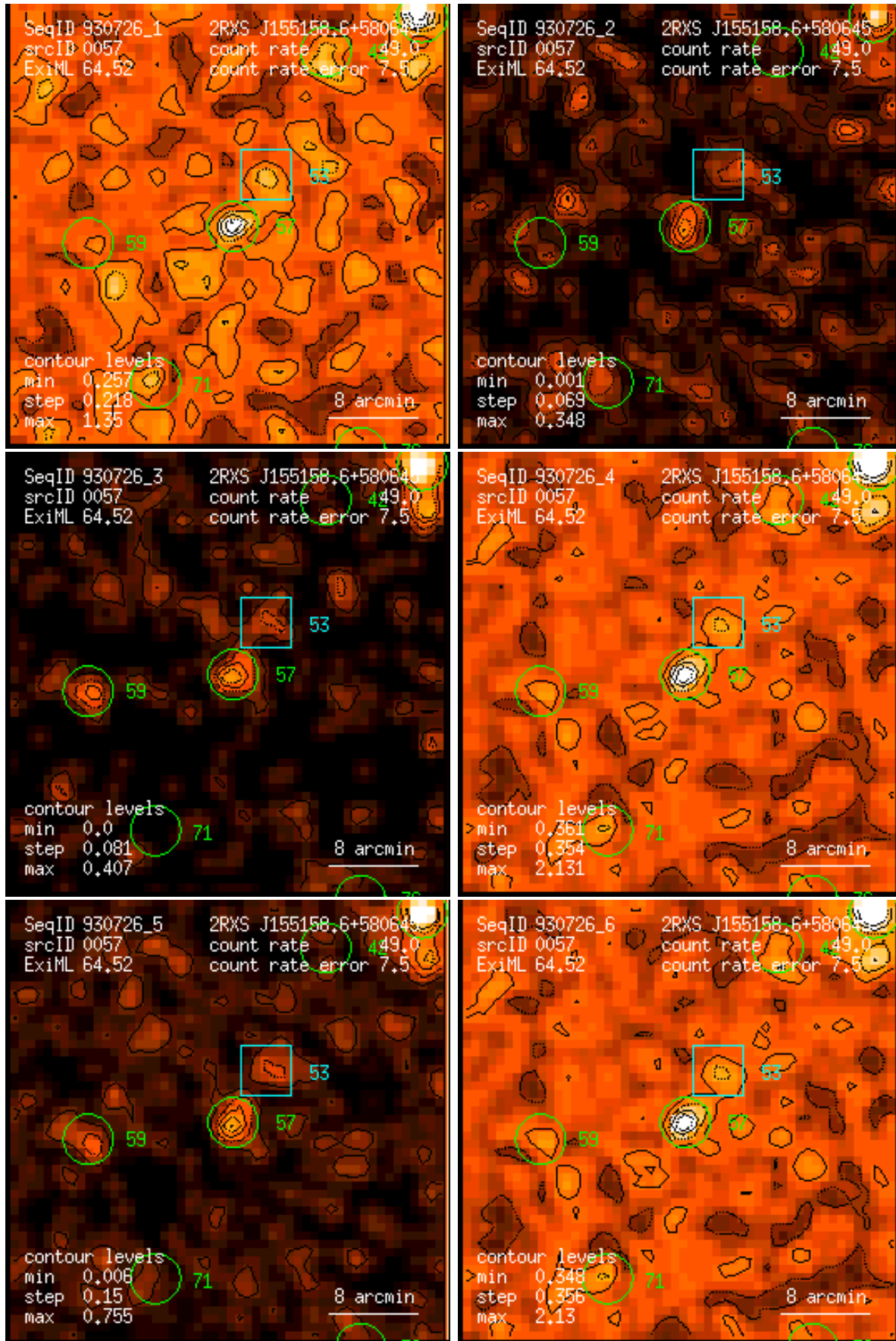
Figure 57: RASS 930726: detection 0057: band rate images, Gaussian filter: (1) PSPC channels 11 – 41, (2) 52 – 90, (3) 91 – 201, (4) 11 – 235, (5) 52 – 201, (6) 11 – 201. Broad band rates in counts/ks. Band rate contour levels in counts/ks/arcmin 2 .
