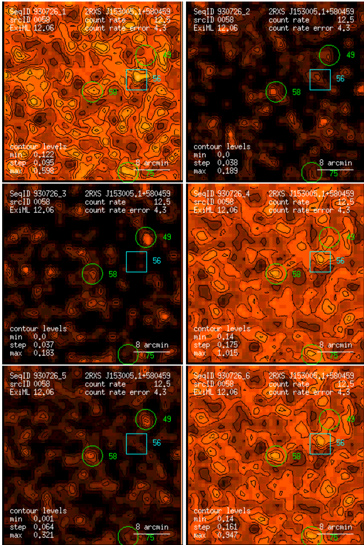
Figure 58: RASS 930726: detection 0058: band rate images, Gaussian filter: (1) PSPC channels 11 – 41, (2) 52 – 90, (3) 91 – 201, (4) 11 – 235, (5) 52 – 201, (6) 11 – 201. Broad band rates in counts/ks. Band rate contour levels in counts/ks/arcmin 2 .
