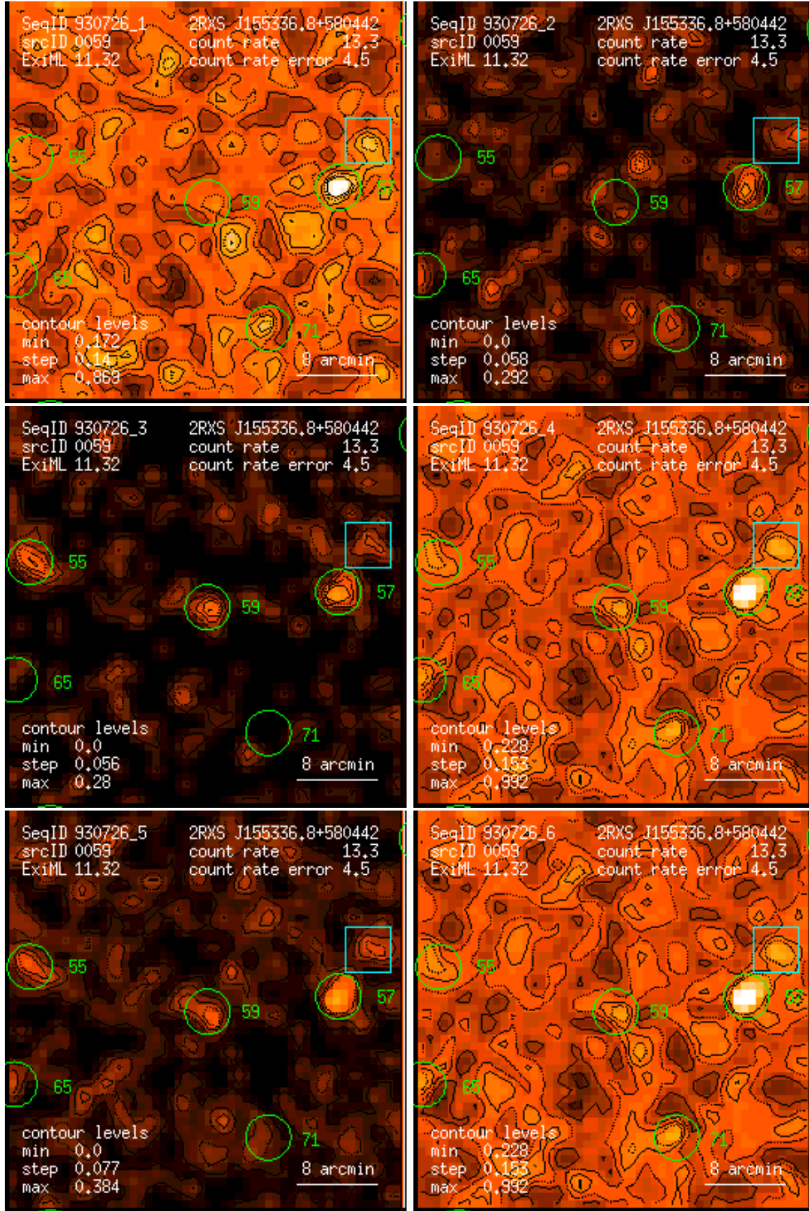
Figure 59: RASS 930726: detection 0059: band rate images, Gaussian filter: (1) PSPC channels 11 – 41, (2) 52 – 90, (3) 91 – 201, (4) 11 – 235, (5) 52 – 201, (6) 11 – 201. Broad band rates in counts/ks. Band rate contour levels in counts/ks/arcmin 2 .
