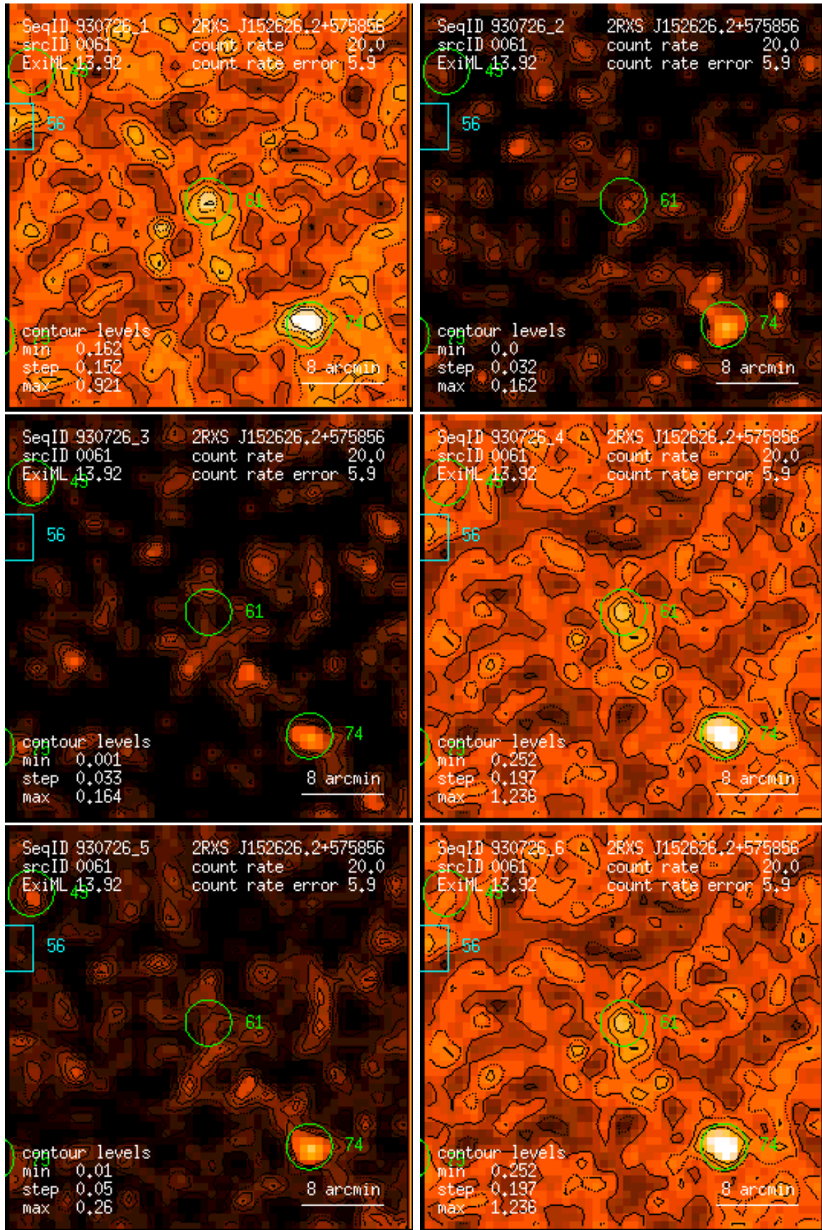
Figure 61: RASS 930726: detection 0061: band rate images, Gaussian filter: (1) PSPC channels 11 – 41, (2) 52 – 90, (3) 91 – 201, (4) 11 – 235, (5) 52 – 201, (6) 11 – 201. Broad band rates in counts/ks. Band rate contour levels in counts/ks/arcmin 2 .
