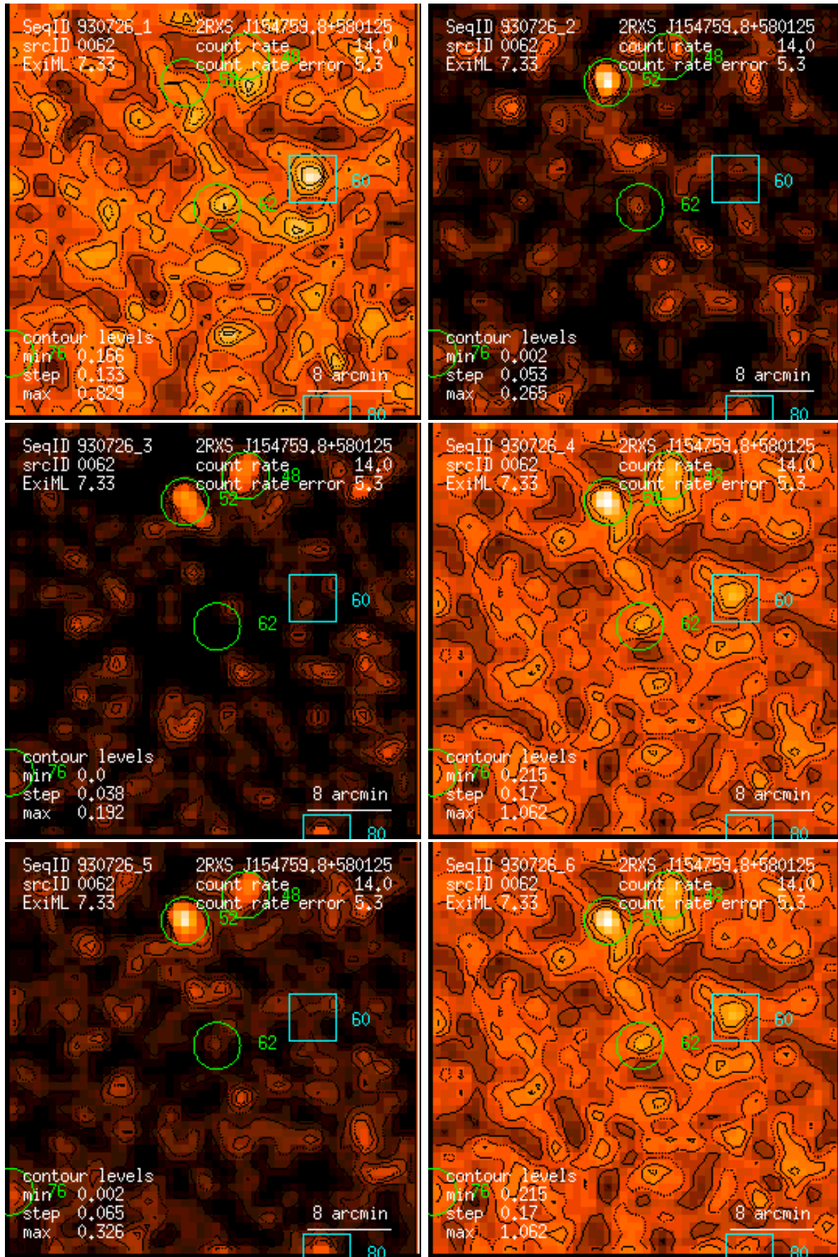
Figure 62: RASS 930726: detection 0062: band rate images, Gaussian filter: (1) PSPC channels 11 – 41, (2) 52 – 90, (3) 91 – 201, (4) 11 – 235, (5) 52 – 201, (6) 11 – 201. Broad band rates in counts/ks. Band rate contour levels in counts/ks/arcmin 2 .
