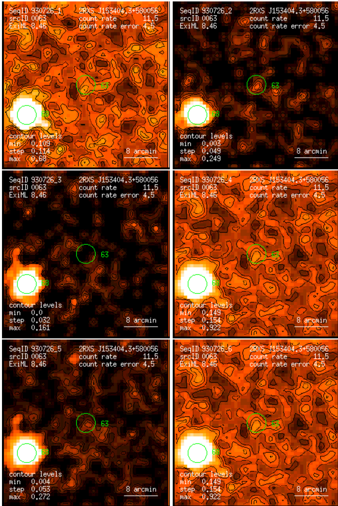
Figure 63: RASS 930726: detection 0063: band rate images, Gaussian filter: (1) PSPC channels 11 – 41, (2) 52 – 90, (3) 91 – 201, (4) 11 – 235, (5) 52 – 201, (6) 11 – 201. Broad band rates in counts/ks. Band rate contour levels in counts/ks/arcmin 2 .
