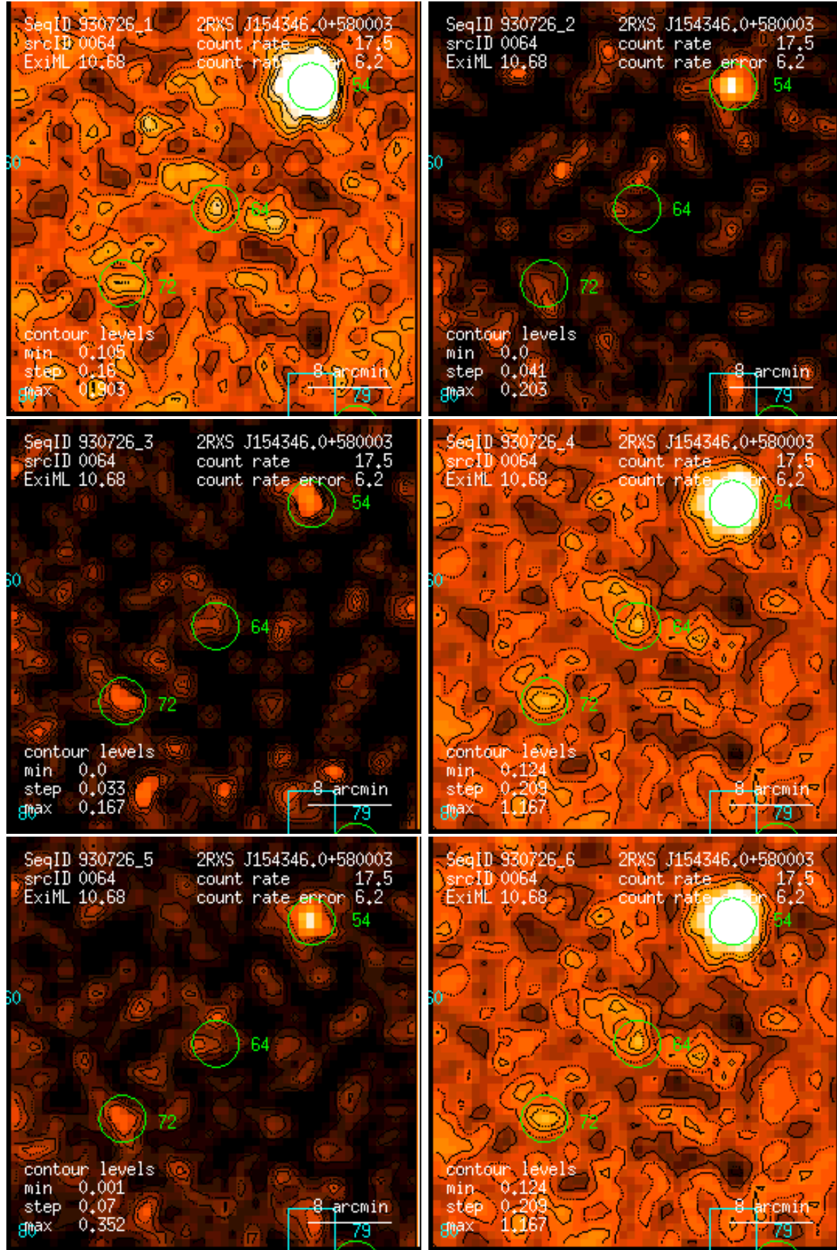
Figure 64: RASS 930726: detection 0064: band rate images, Gaussian filter: (1) PSPC channels 11 – 41, (2) 52 – 90, (3) 91 – 201, (4) 11 – 235, (5) 52 – 201, (6) 11 – 201. Broad band rates in counts/ks. Band rate contour levels in counts/ks/arcmin 2 .
