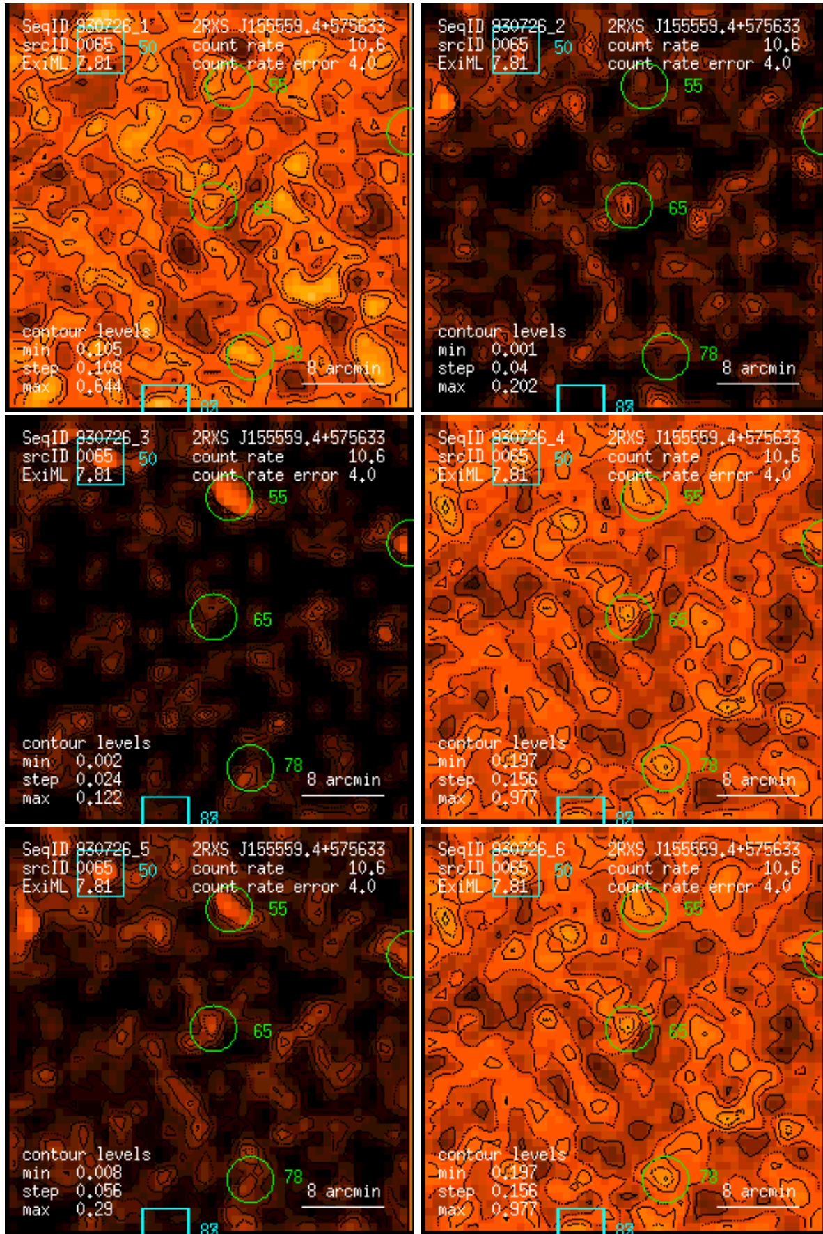
Figure 65: RASS 930726: detection 0065: band rate images, Gaussian filter: (1) PSPC channels 11 – 41, (2) 52 – 90, (3) 91 – 201, (4) 11 – 235, (5) 52 – 201, (6) 11 – 201. Broad band rates in counts/ks. Band rate contour levels in counts/ks/arcmin 2 .
