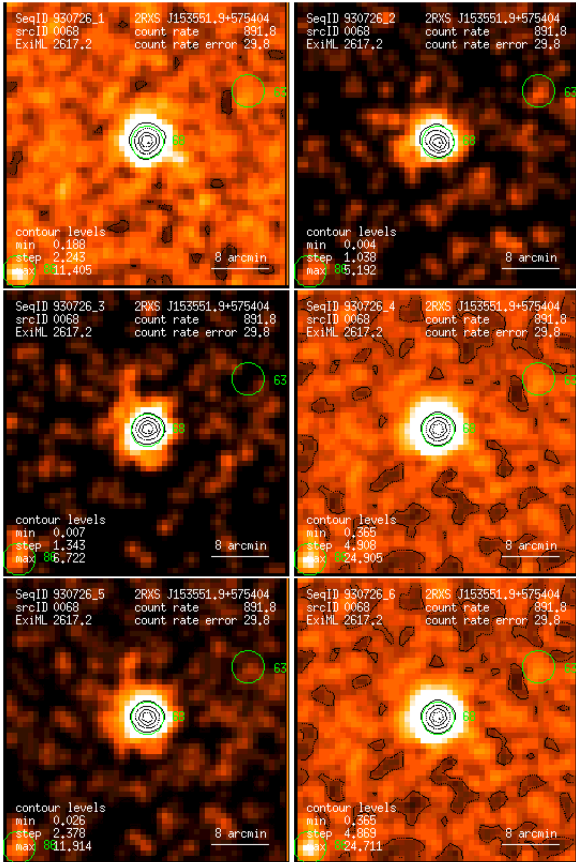
Figure 68: RASS 930726: detection 0068: band rate images, Gaussian filter: (1) PSPC channels 11 – 41, (2) 52 – 90, (3) 91 – 201, (4) 11 – 235, (5) 52 – 201, (6) 11 – 201. Broad band rates in counts/ks. Band rate contour levels in counts/ks/arcmin 2 .
