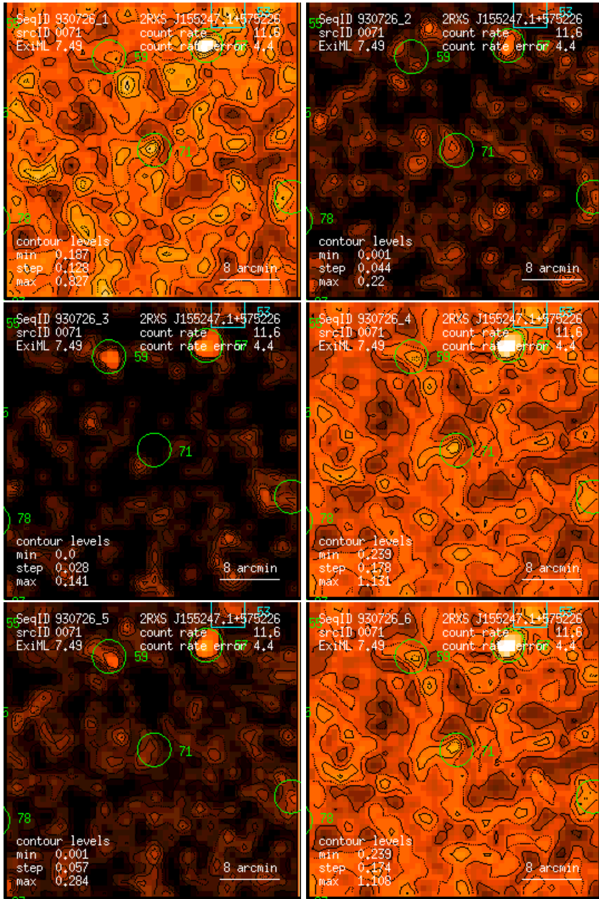
Figure 71: RASS 930726: detection 0071: band rate images, Gaussian filter: (1) PSPC channels 11 – 41, (2) 52 – 90, (3) 91 – 201, (4) 11 – 235, (5) 52 – 201, (6) 11 – 201. Broad band rates in counts/ks. Band rate contour levels in counts/ks/arcmin 2 .
