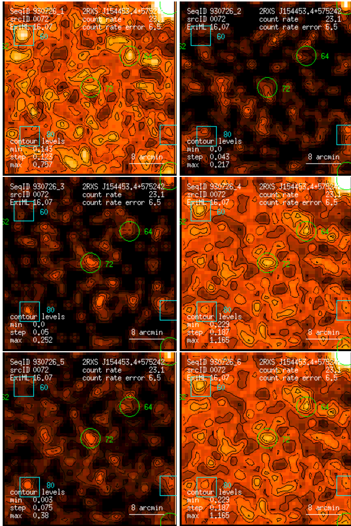
Figure 72: RASS 930726: detection 0072: band rate images, Gaussian filter: (1) PSPC channels 11 – 41, (2) 52 – 90, (3) 91 – 201, (4) 11 – 235, (5) 52 – 201, (6) 11 – 201. Broad band rates in counts/ks. Band rate contour levels in counts/ks/arcmin 2 .
