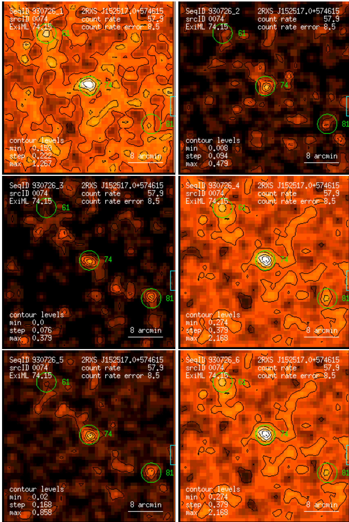
Figure 74: RASS 930726: detection 0074: band rate images, Gaussian filter: (1) PSPC channels 11 – 41, (2) 52 – 90, (3) 91 – 201, (4) 11 – 235, (5) 52 – 201, (6) 11 – 201. Broad band rates in counts/ks. Band rate contour levels in counts/ks/arcmin 2 .
