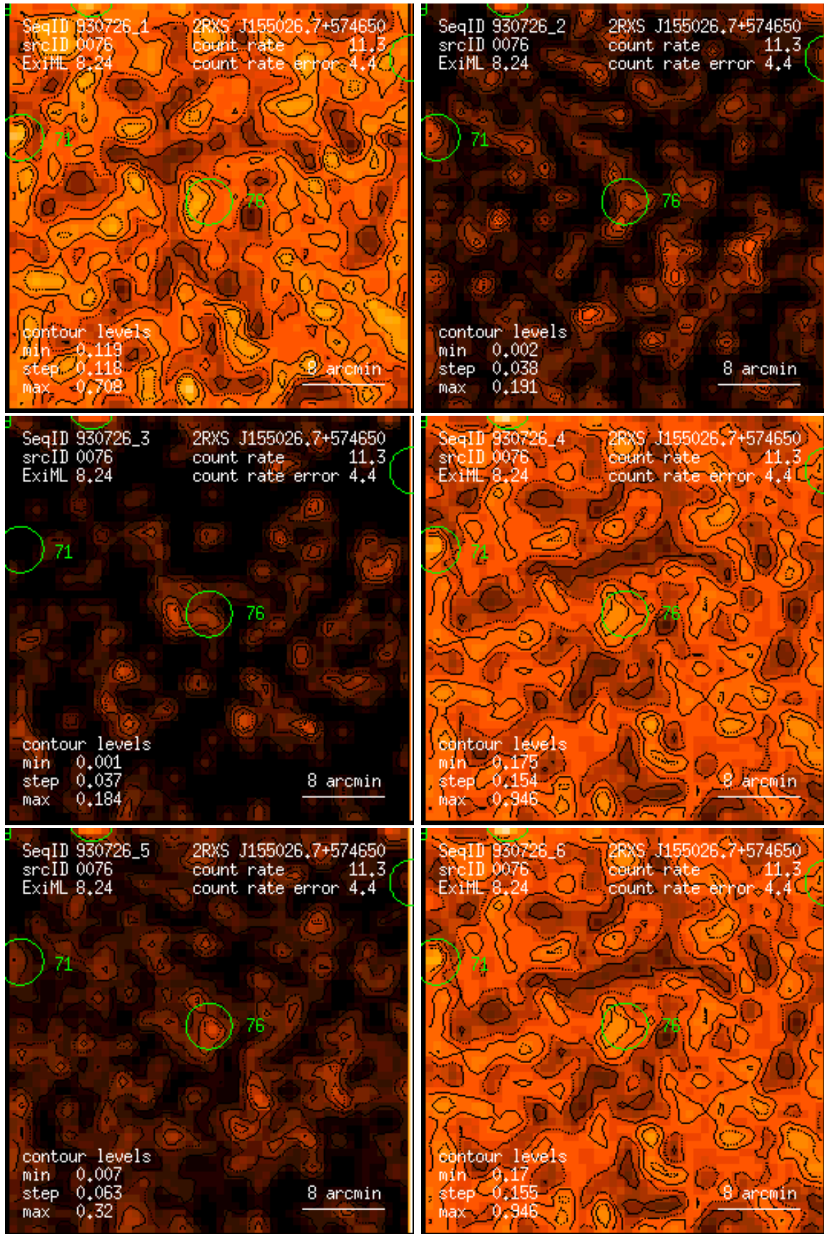
Figure 76: RASS 930726: detection 0076: band rate images, Gaussian filter: (1) PSPC channels 11 – 41, (2) 52 – 90, (3) 91 – 201, (4) 11 – 235, (5) 52 – 201, (6) 11 – 201. Broad band rates in counts/ks. Band rate contour levels in counts/ks/arcmin 2 .
