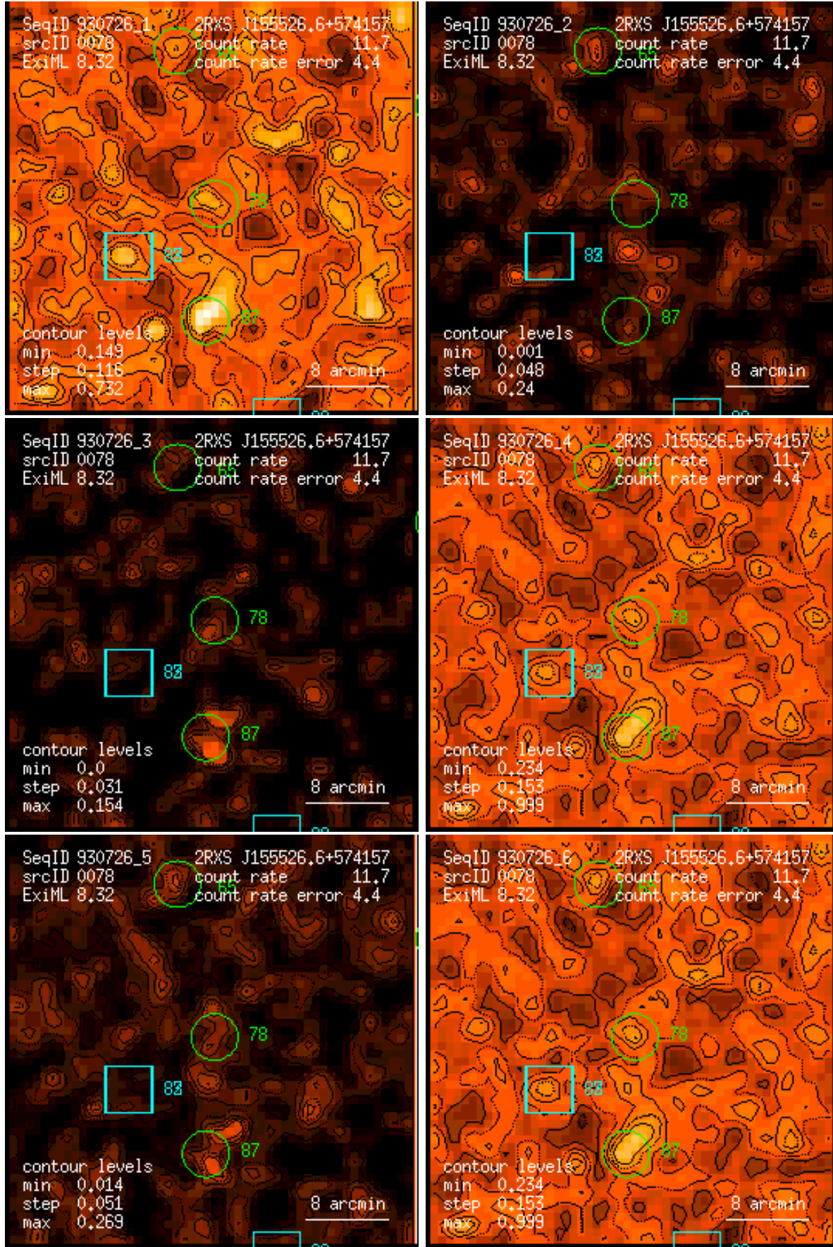
Figure 78: RASS 930726: detection 0078: band rate images, Gaussian filter: (1) PSPC channels 11 – 41, (2) 52 – 90, (3) 91 – 201, (4) 11 – 235, (5) 52 – 201, (6) 11 – 201. Broad band rates in counts/ks. Band rate contour levels in counts/ks/arcmin 2 .
