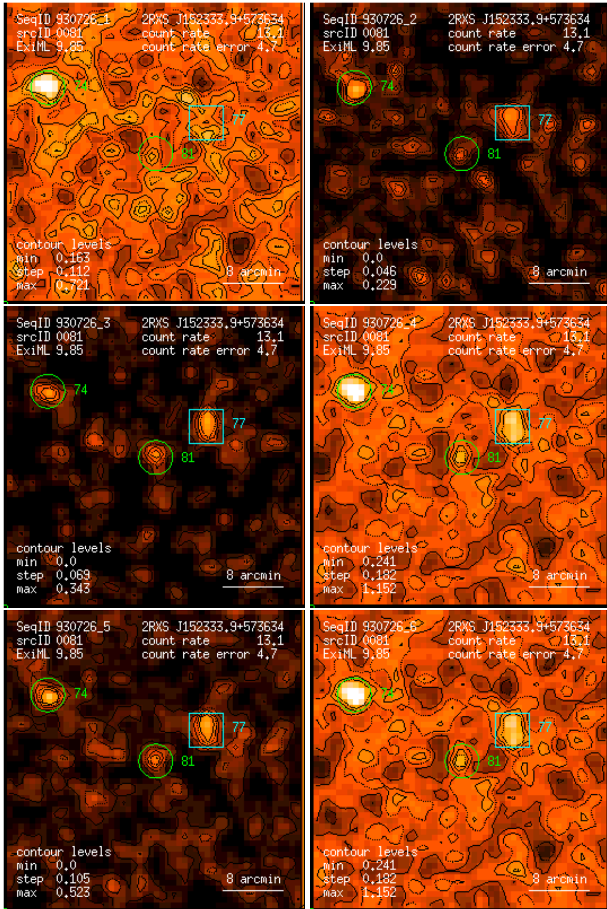
Figure 81: RASS 930726: detection 0081: band rate images, Gaussian filter: (1) PSPC channels 11 – 41, (2) 52 – 90, (3) 91 – 201, (4) 11 – 235, (5) 52 – 201, (6) 11 – 201. Broad band rates in counts/ks. Band rate contour levels in counts/ks/arcmin 2 .
