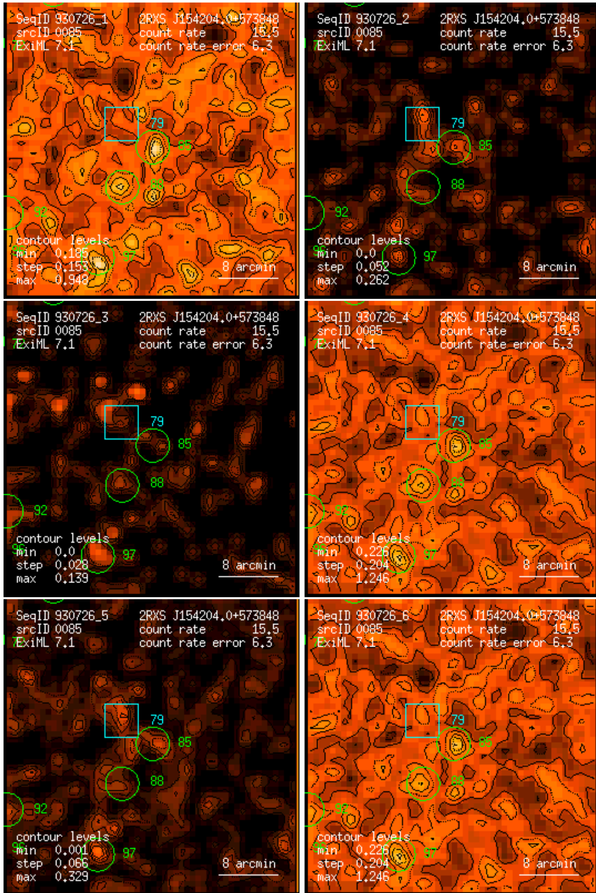
Figure 85: RASS 930726: detection 0085: band rate images, Gaussian filter: (1) PSPC channels 11 – 41, (2) 52 – 90, (3) 91 – 201, (4) 11 – 235, (5) 52 – 201, (6) 11 – 201. Broad band rates in counts/ks. Band rate contour levels in counts/ks/arcmin 2 .
