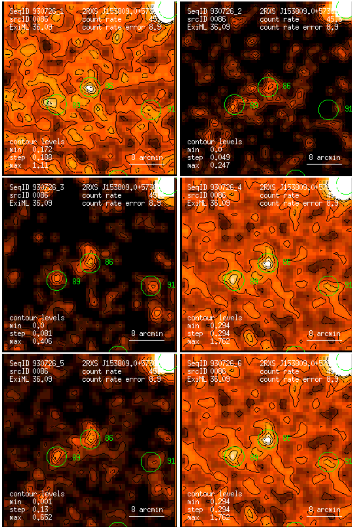
Figure 86: RASS 930726: detection 0086: band rate images, Gaussian filter: (1) PSPC channels 11 – 41, (2) 52 – 90, (3) 91 – 201, (4) 11 – 235, (5) 52 – 201, (6) 11 – 201. Broad band rates in counts/ks. Band rate contour levels in counts/ks/arcmin 2 .
