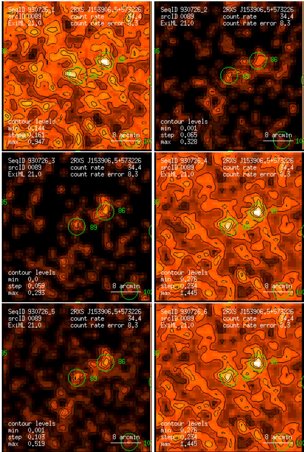
Figure 89: RASS 930726: detection 0089: band rate images, Gaussian filter: (1) PSPC channels 11 – 41, (2) 52 – 90, (3) 91 – 201, (4) 11 – 235, (5) 52 – 201, (6) 11 – 201. Broad band rates in counts/ks. Band rate contour levels in counts/ks/arcmin 2 .
