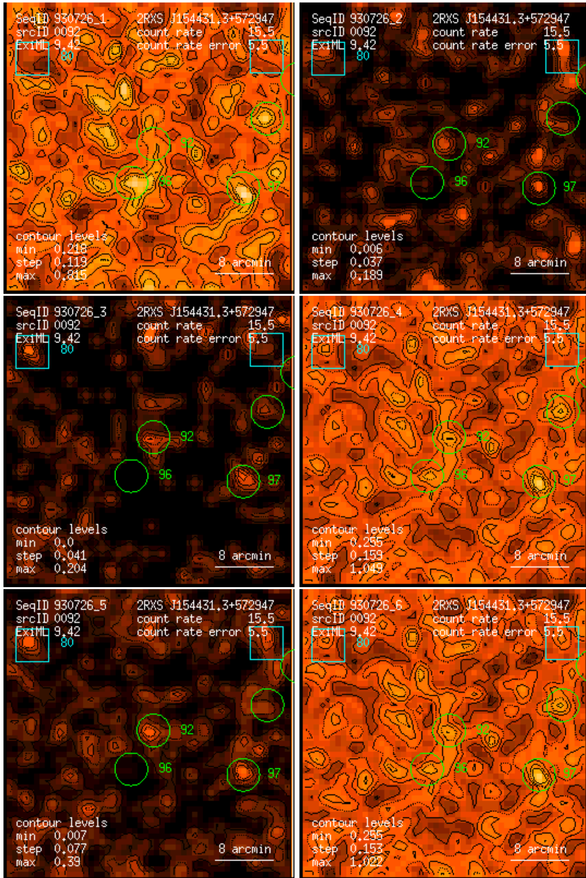
Figure 92: RASS 930726: detection 0092: band rate images, Gaussian filter: (1) PSPC channels 11 – 41, (2) 52 – 90, (3) 91 – 201, (4) 11 – 235, (5) 52 – 201, (6) 11 – 201. Broad band rates in counts/ks. Band rate contour levels in counts/ks/arcmin 2 .
