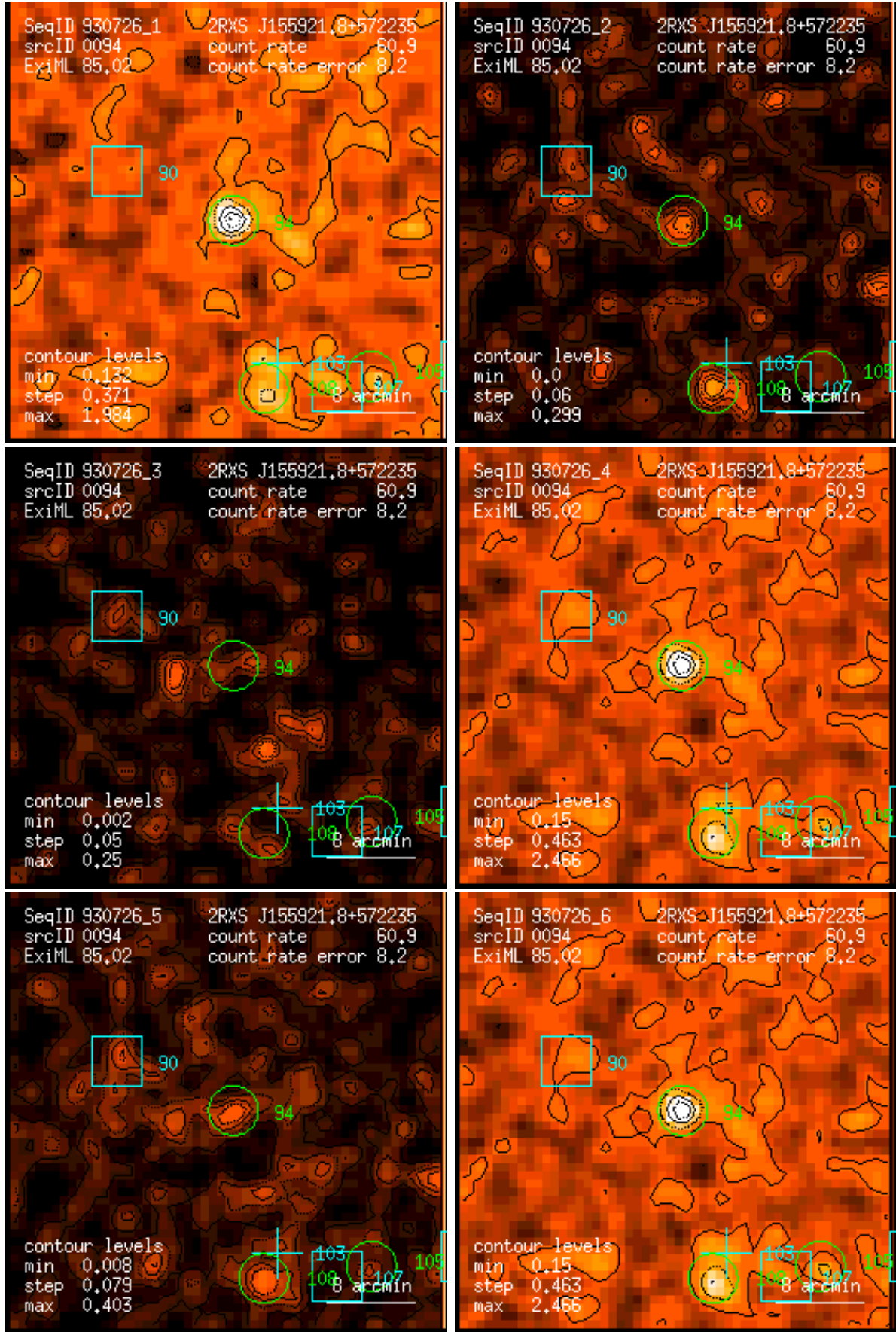
Figure 94: RASS 930726: detection 0094: band rate images, Gaussian filter: (1) PSPC channels 11 – 41, (2) 52 – 90, (3) 91 – 201, (4) 11 – 235, (5) 52 – 201, (6) 11 – 201. Broad band rates in counts/ks. Band rate contour levels in counts/ks/arcmin 2 .
