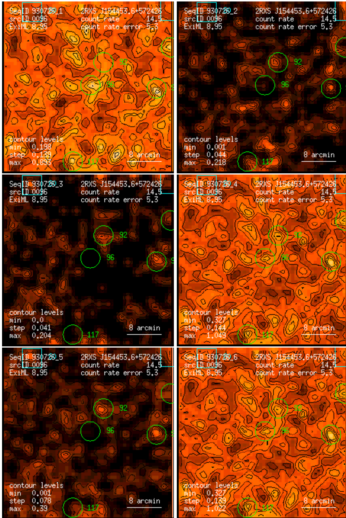
Figure 96: RASS 930726: detection 0096: band rate images, Gaussian filter: (1) PSPC channels 11 – 41, (2) 52 – 90, (3) 91 – 201, (4) 11 – 235, (5) 52 – 201, (6) 11 – 201. Broad band rates in counts/ks. Band rate contour levels in counts/ks/arcmin 2 .
