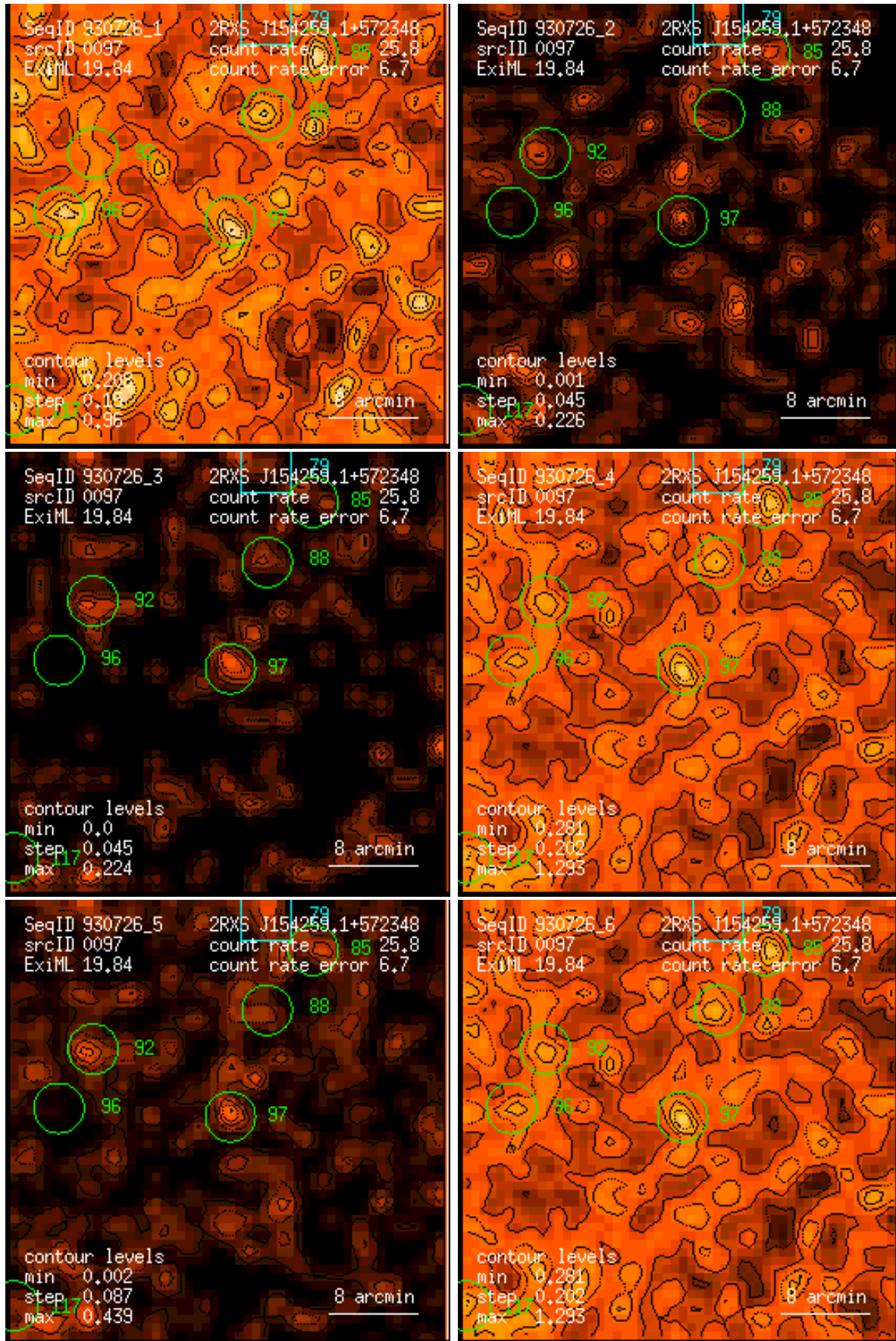
Figure 97: RASS 930726: detection 0097: band rate images, Gaussian filter: (1) PSPC channels 11 – 41, (2) 52 – 90, (3) 91 – 201, (4) 11 – 235, (5) 52 – 201, (6) 11 – 201. Broad band rates in counts/ks. Band rate contour levels in counts/ks/arcmin 2 .
