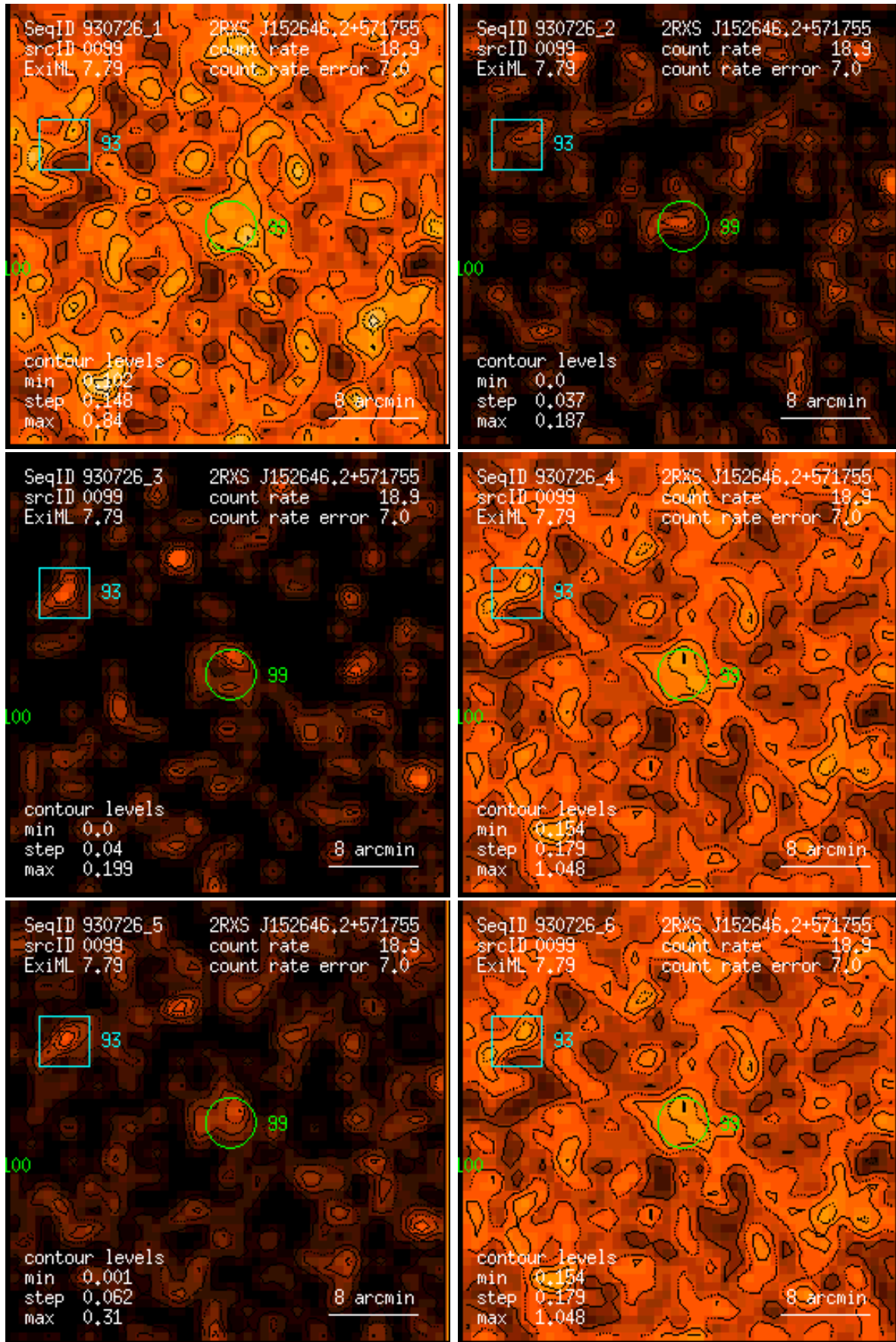
Figure 99: RASS 930726: detection 0099: band rate images, Gaussian filter: (1) PSPC channels 11 – 41, (2) 52 – 90, (3) 91 – 201, (4) 11 – 235, (5) 52 – 201, (6) 11 – 201. Broad band rates in counts/ks. Band rate contour levels in counts/ks/arcmin 2 .
