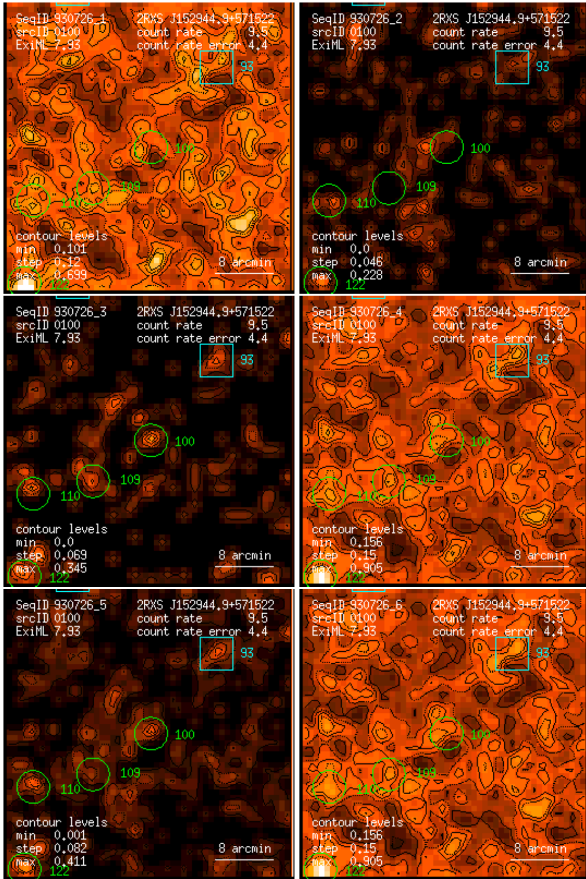
Figure 100: RASS 930726: detection 0100: band rate images, Gaussian filter: (1) PSPC channels 11 – 41, (2) 52 – 90, (3) 91 – 201, (4) 11 – 235, (5) 52 – 201, (6) 11 – 201. Broad band rates in counts/ks. Band rate contour levels in counts/ks/arcmin 2 .
