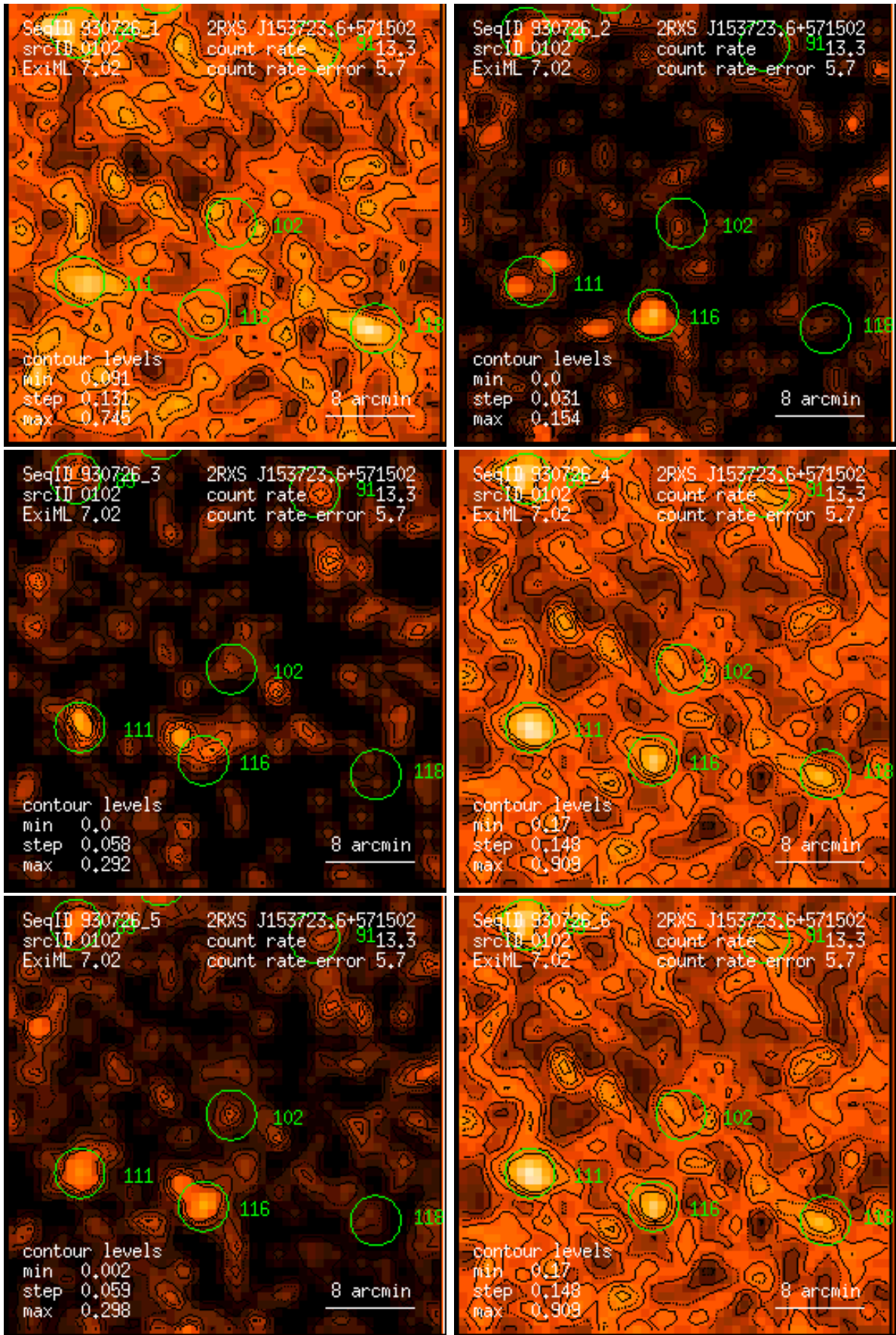
Figure 102: RASS 930726: detection 0102: band rate images, Gaussian filter: (1) PSPC channels 11 – 41, (2) 52 – 90, (3) 91 – 201, (4) 11 – 235, (5) 52 – 201, (6) 11 – 201. Broad band rates in counts/ks. Band rate contour levels in counts/ks/arcmin 2 .
