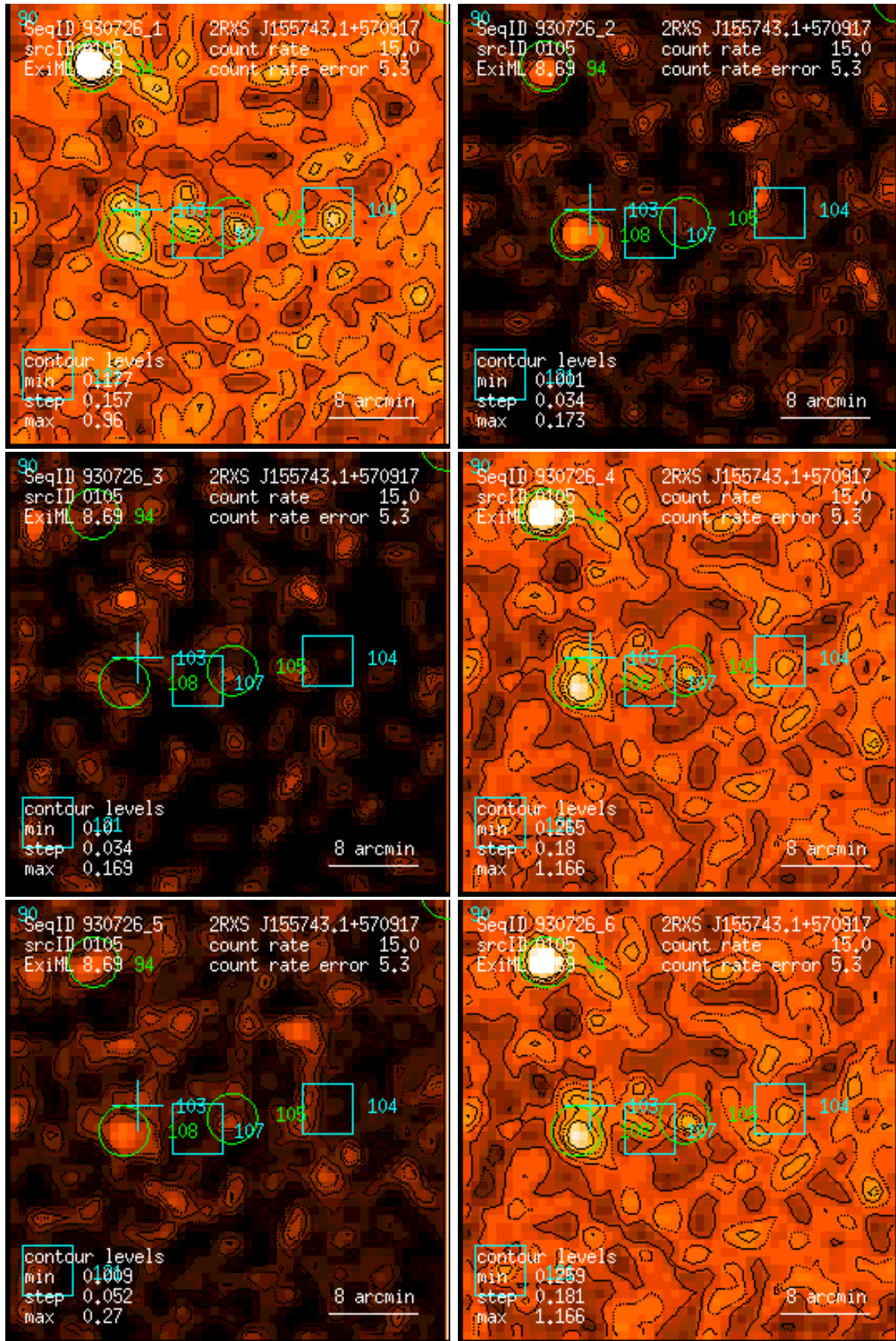
Figure 105: RASS 930726: detection 0105: band rate images, Gaussian filter: (1) PSPC channels 11 – 41, (2) 52 – 90, (3) 91 – 201, (4) 11 – 235, (5) 52 – 201, (6) 11 – 201. Broad band rates in counts/ks. Band rate contour levels in counts/ks/arcmin 2 .
