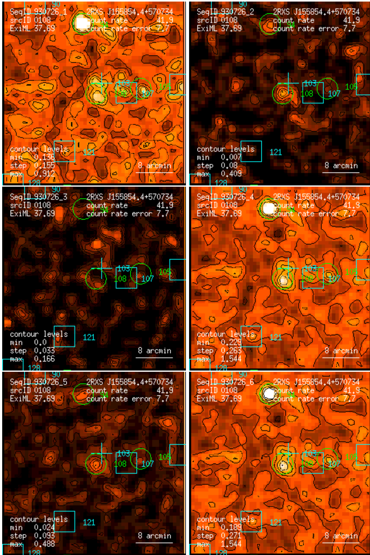
Figure 108: RASS 930726: detection 0108: band rate images, Gaussian filter: (1) PSPC channels 11 – 41, (2) 52 – 90, (3) 91 – 201, (4) 11 – 235, (5) 52 – 201, (6) 11 – 201. Broad band rates in counts/ks. Band rate contour levels in counts/ks/arcmin 2 .
