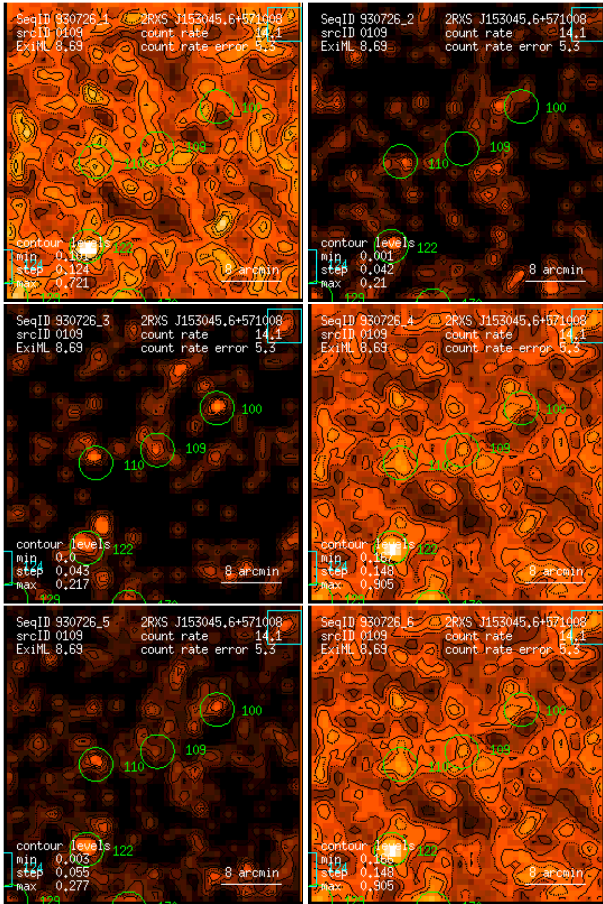
Figure 109: RASS 930726: detection 0109: band rate images, Gaussian filter: (1) PSPC channels 11 – 41, (2) 52 – 90, (3) 91 – 201, (4) 11 – 235, (5) 52 – 201, (6) 11 – 201. Broad band rates in counts/ks. Band rate contour levels in counts/ks/arcmin 2 .
