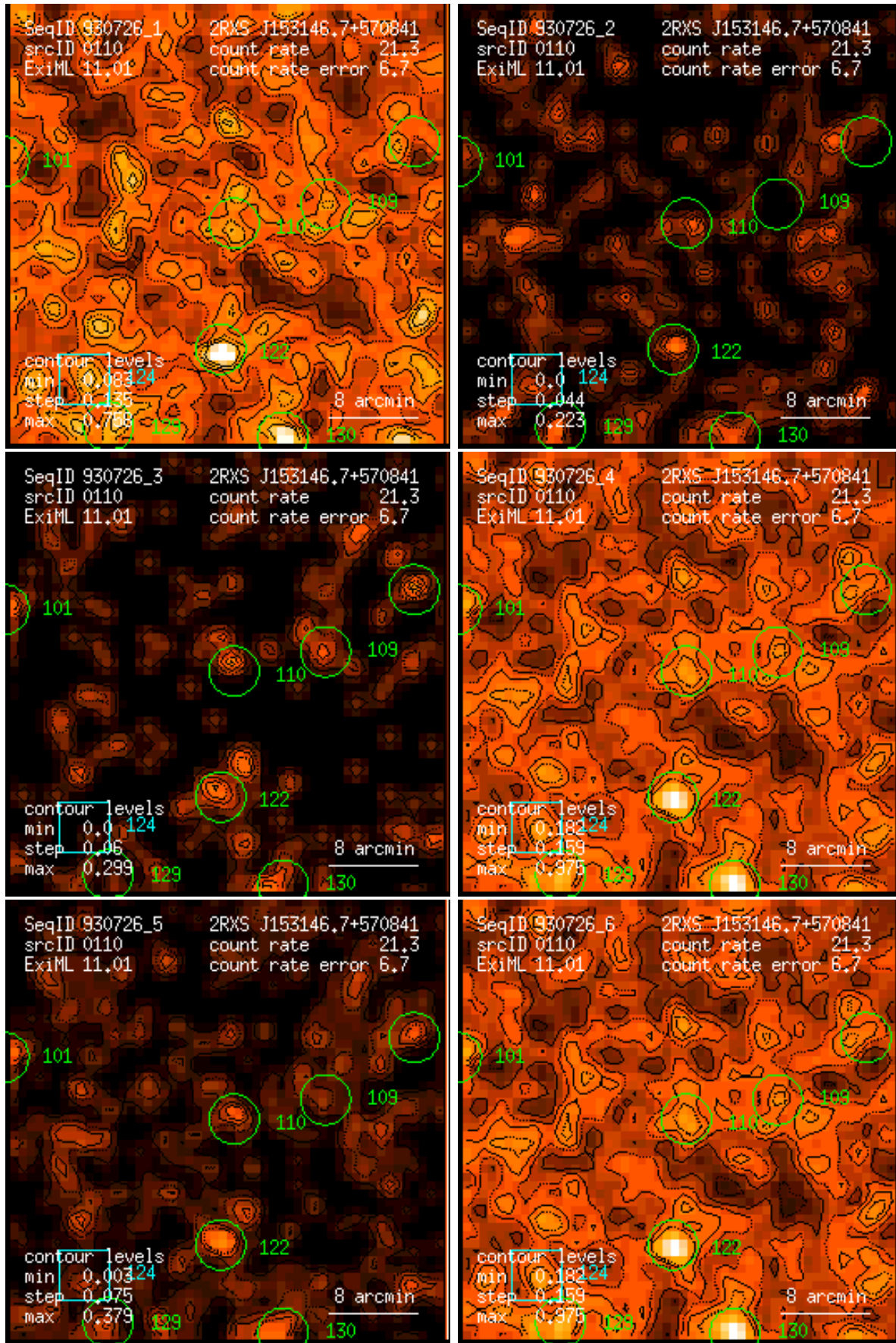
Figure 110: RASS 930726: detection 0110: band rate images, Gaussian filter: (1) PSPC channels 11 – 41, (2) 52 – 90, (3) 91 – 201, (4) 11 – 235, (5) 52 – 201, (6) 11 – 201. Broad band rates in counts/ks. Band rate contour levels in counts/ks/arcmin 2 .
