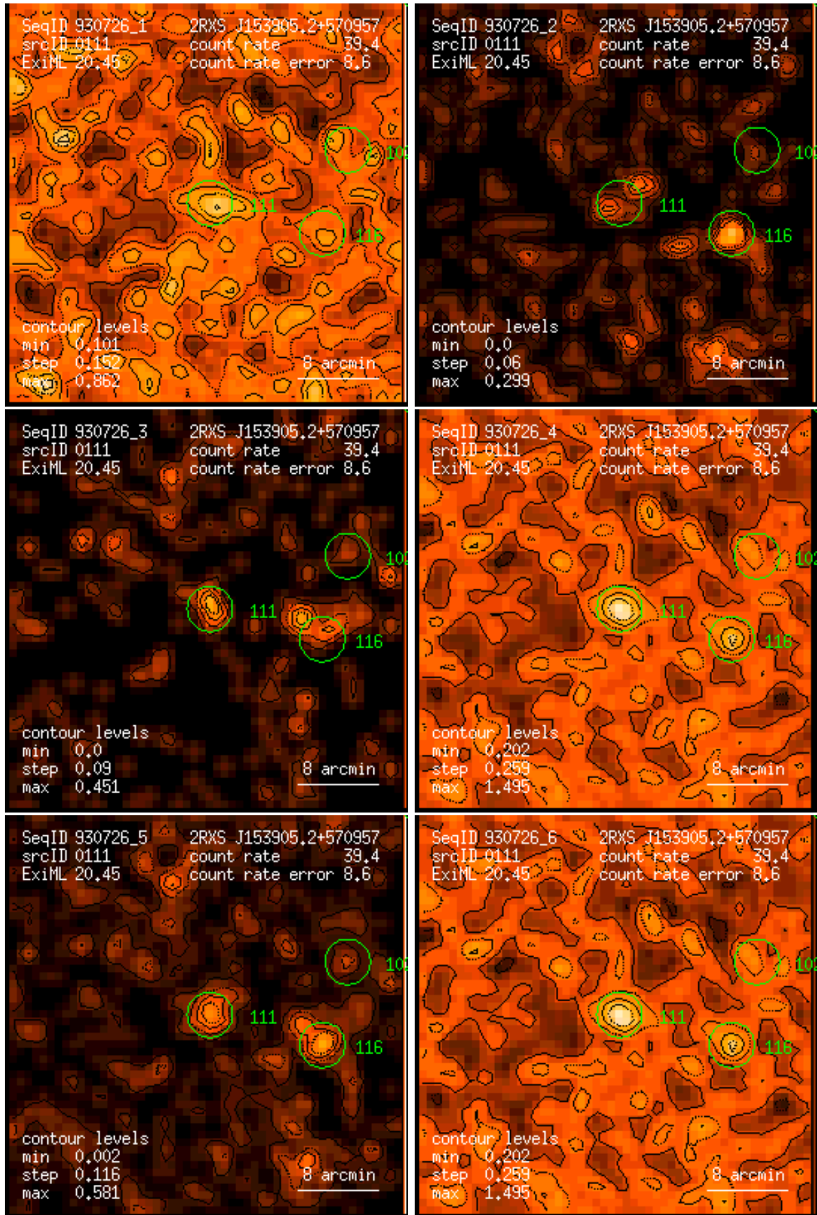
Figure 111: RASS 930726: detection 0111: band rate images, Gaussian filter: (1) PSPC channels 11 – 41, (2) 52 – 90, (3) 91 – 201, (4) 11 – 235, (5) 52 – 201, (6) 11 – 201. Broad band rates in counts/ks. Band rate contour levels in counts/ks/arcmin 2 .
