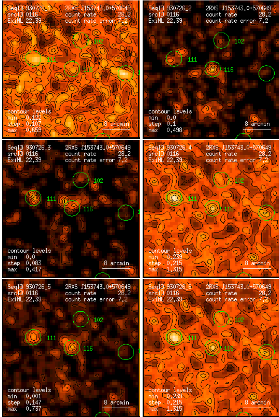
Figure 116: RASS 930726: detection 0116: band rate images, Gaussian filter: (1) PSPC channels 11 – 41, (2) 52 – 90, (3) 91 – 201, (4) 11 – 235, (5) 52 – 201, (6) 11 – 201. Broad band rates in counts/ks. Band rate contour levels in counts/ks/arcmin 2 .
